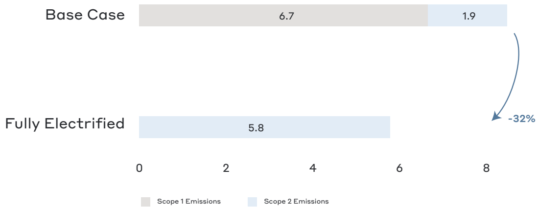
Figure 2 – GHG emissions per TEU in a case study where the container terminal had about 80 percent of the emissions related to diesel-fuelled equipment and planned to switch to fully electric operations.
