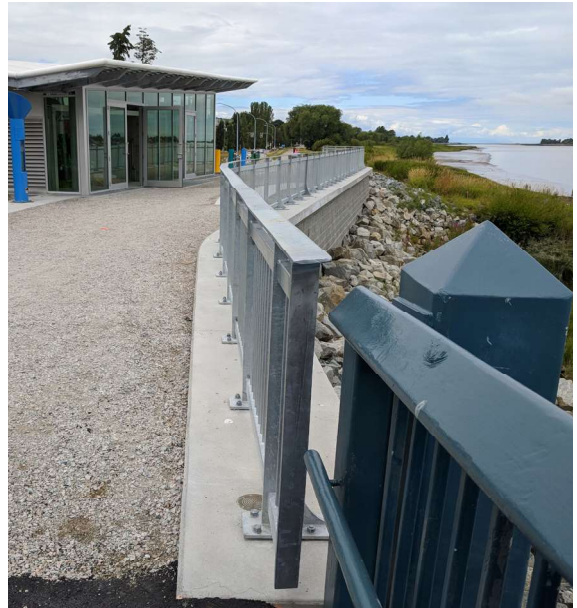
Dike upgrades along the foreshore were specifically designed to keep all disturbances above the high water level, helping to preserve the natural habitat.
