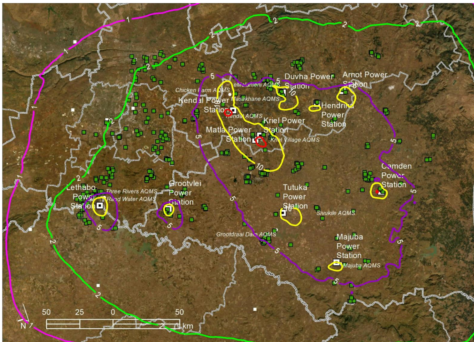
Figure 6-29: Predicted annual average PM 10 concentrations in µg/m 3 for Scenario A (2025) (NAAQS Limit is 40 µg/m 3 )
