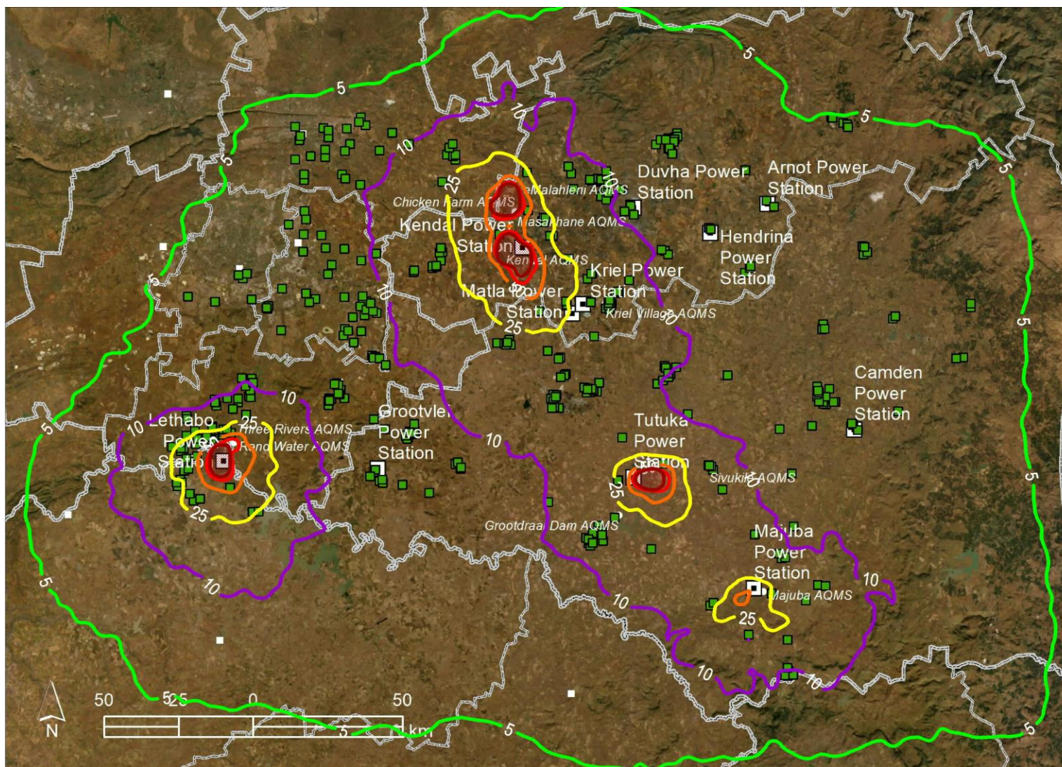
Figure 6-36: Predicted 99 th percentile of the 24-hour PM 10 concentrations in µg/m 3 for Scenario D (MES) (NAAQS Limit is 75 µg/m 3 )
