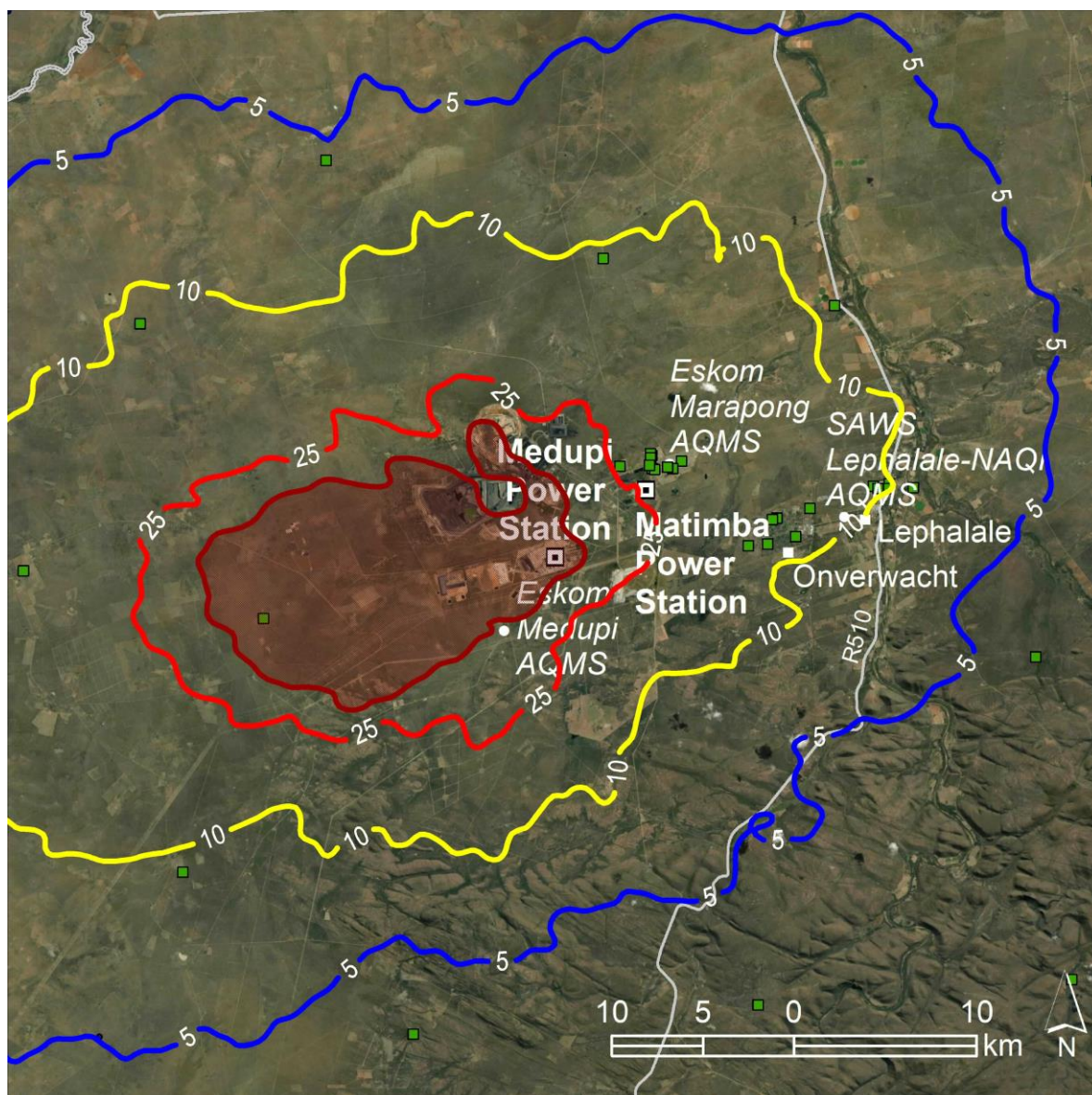
Figure 7-42: Predicted 99 th percentile of the 24-hour PM 2.5 concentrations in µg/m 3 resulting from emissions from Medupi: Scenario B (2031) (NAAQS limit 25 ug/m 3 )
