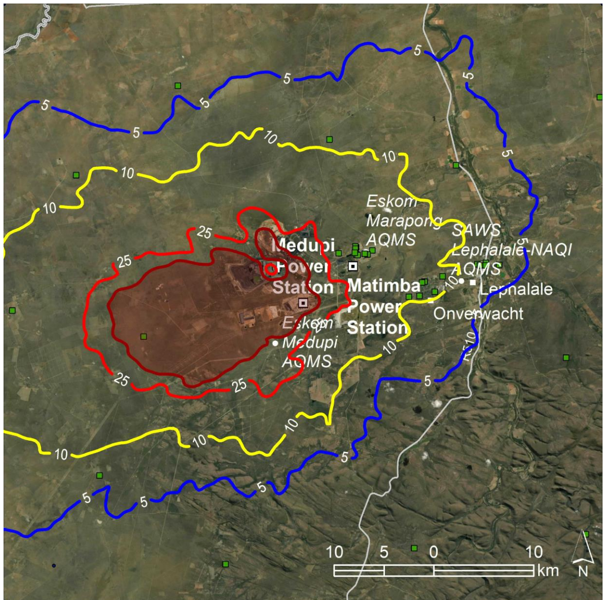
Figure 7-46: Predicted 99 th percentile of the 24-hour PM 2.5 concentrations in µg/m 3 resulting from emissions from Medupi: Scenario D (MES) (NAAQS limit 25 ug/m 3 )
