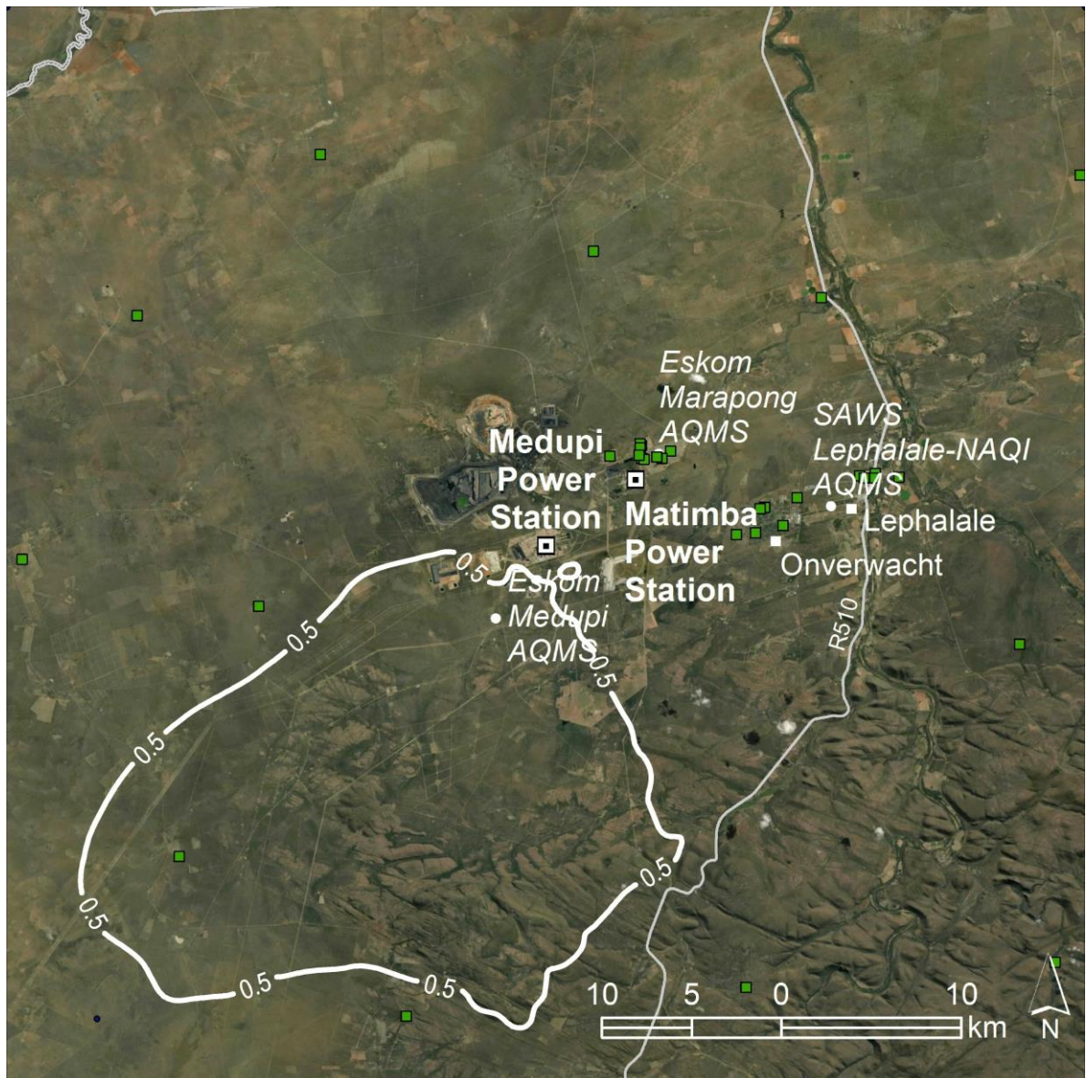
Figure 7-17: Predicted annual average NO 2 concentrations in µg/m 3 resulting from emissions from Medupi: Scenario 1 (Current) (NAAQS limit 40 ug/m 3 )
