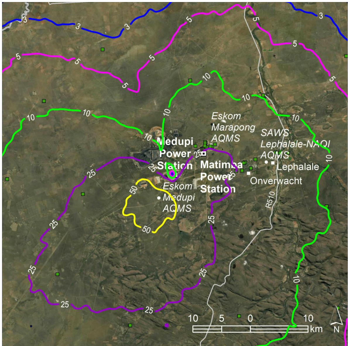
Figure 7-20: Predicted 99 th percentile 1-hour NO 2 concentrations in µg/m 3 resulting from emissions from Medupi: Scenario A (2025) (NAAQS limit 200 µg/m 3 )
