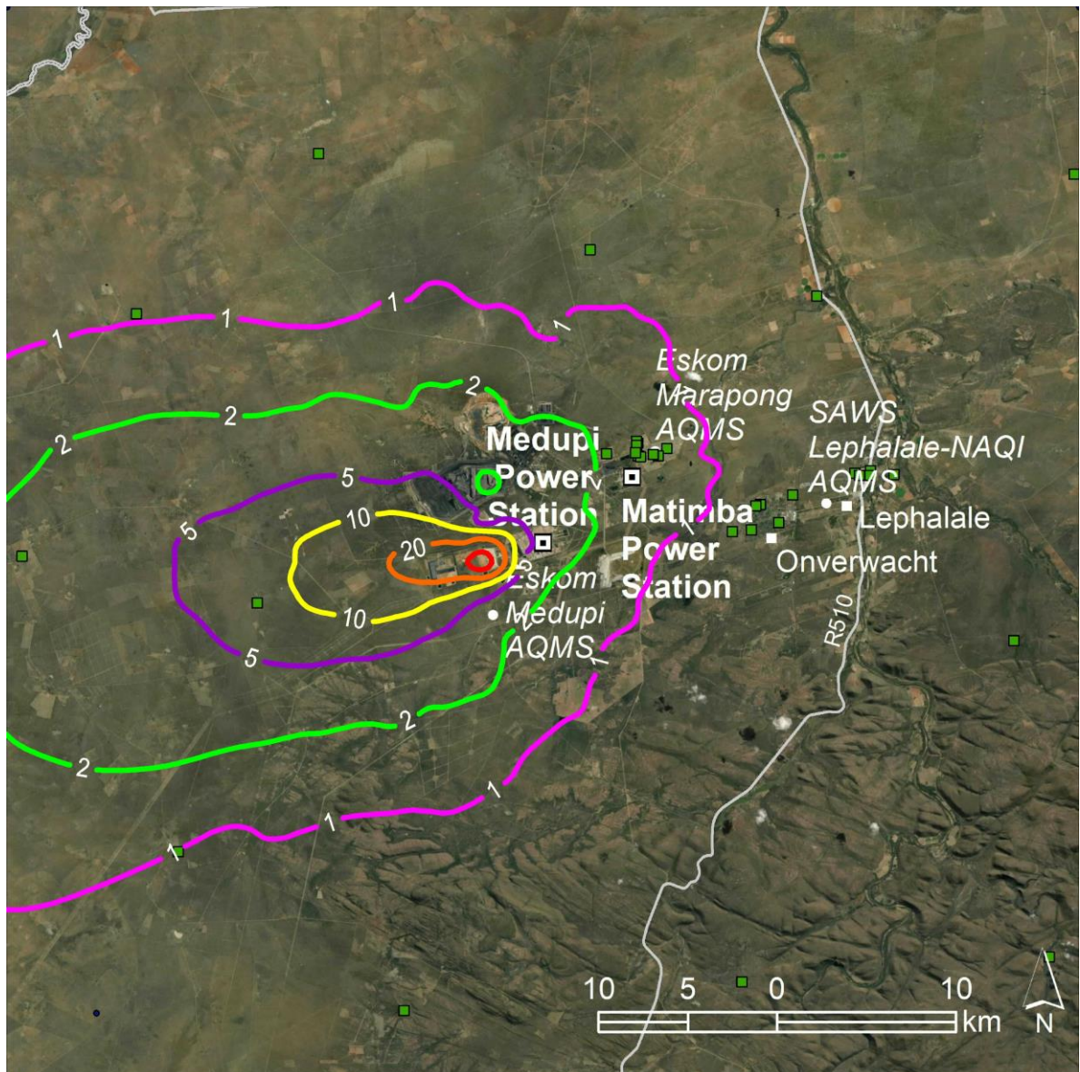
Figure 7-31: Predicted annual average PM 10 concentrations in µg/m 3 resulting from emissions from Medupi: Scenario B (2031) (NAAQS limit 40 ug/m 3 )
