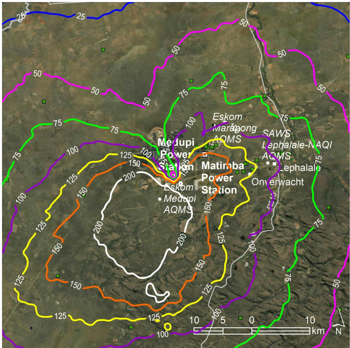
Figure 7-7: Predicted 99 th percentile 1-hour SO 2 concentrations in µg/m 3 resulting from emissions from Medupi: Scenario A (2025) (NAAQS limit 350 ug/m 3 )
