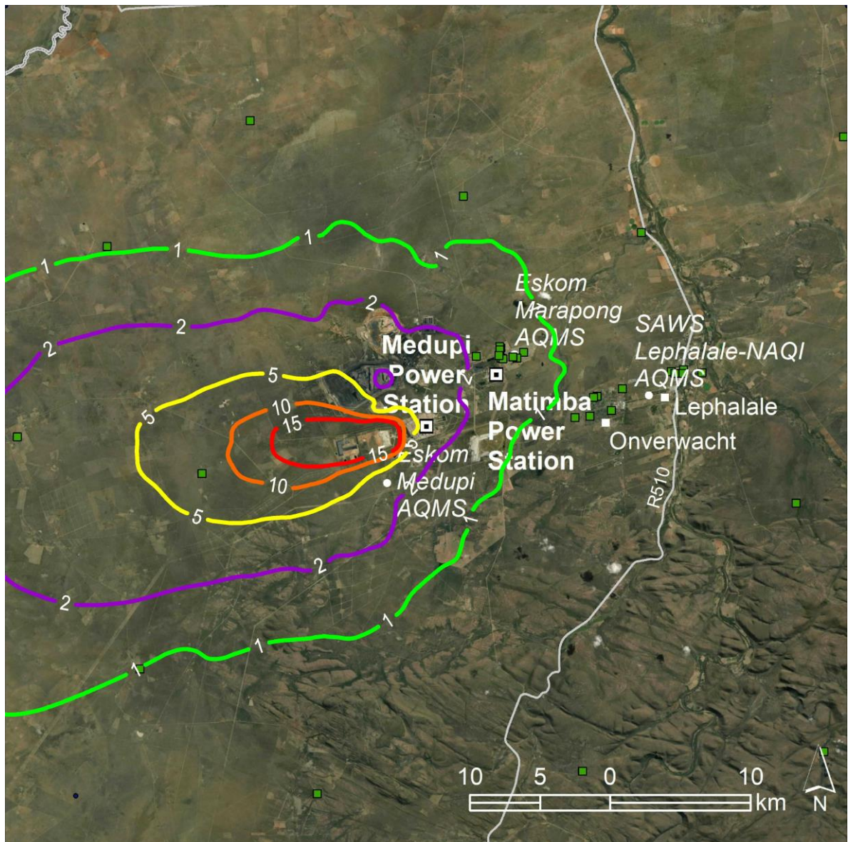
Figure 7-41: Predicted annual average PM 2.5 concentrations in µg/m 3 resulting from emissions from Medupi: Scenario B (2031) (NAAQS limit 15 ug/m 3 )
