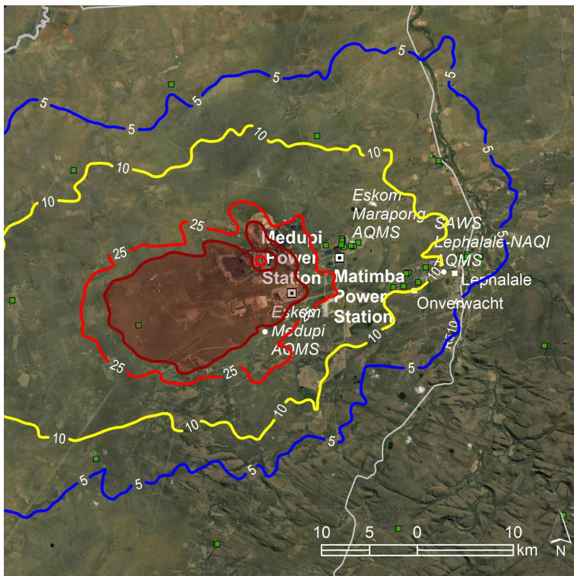
Figure 7-44: Predicted 99 th percentile of the 24-hour PM 2.5 concentrations in µg/m 3 resulting from emissions from Medupi: Scenario C (2036) (NAAQS limit 25 ug/m 3 )
