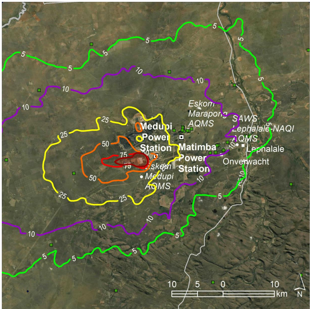
Figure 7-34: Predicted 99 th percentile of the 24-hour PM 10 concentrations in µg/m 3 resulting from emissions from Medupi: Scenario C (2036) (NAAQS limit 75 ug/m 3 )
