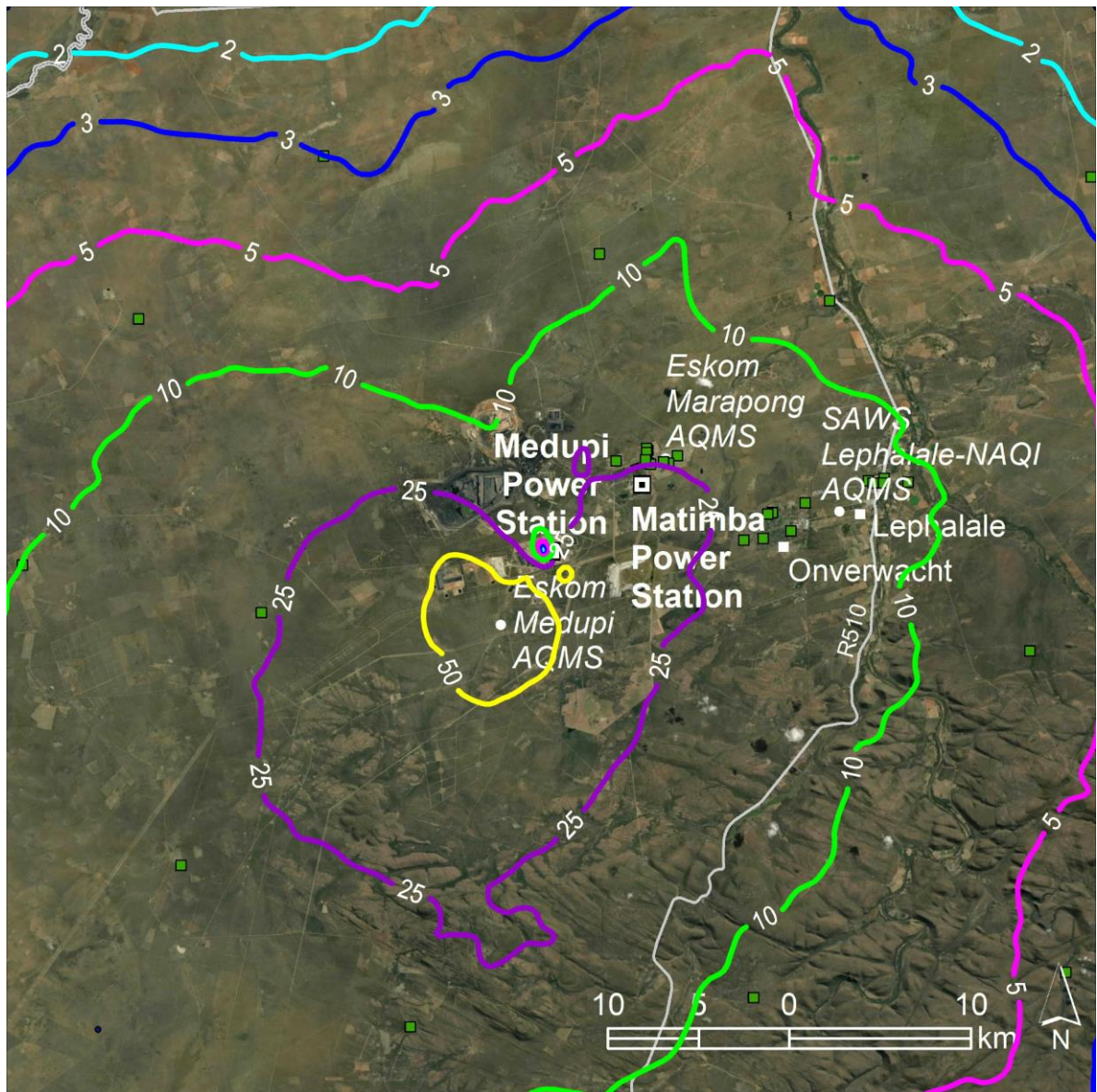
Figure 7-22: Predicted 99 th percentile 1-hour NO 2 concentrations in µg/m 3 resulting from emissions from Medupi: Scenario B (2031) (NAAQS limit 200 µg/m 3 )
