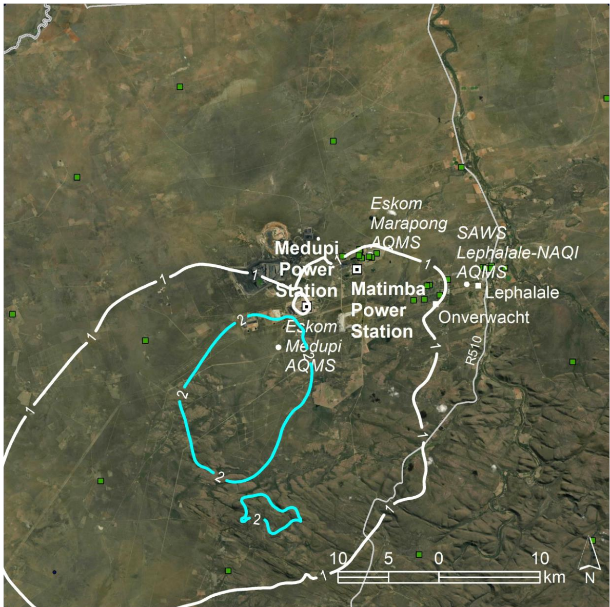
Figure 7-11: Predicted annual average \text{SO}_2 concentrations in \mu\text{g}/\text{m}^3 resulting from emissions from Medupi: Scenario C (2036) (NAAQS limit 50 \mu\text{g}/\text{m}^3 )
