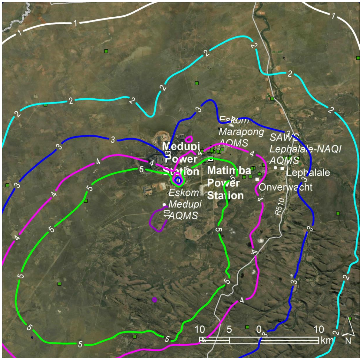
Figure 7-5: Predicted annual average \text{SO}_2 concentrations in \mu\text{g}/\text{m}^3 resulting from emissions from Medupi: Scenario A (2025) (NAAQS limit 50 \mu\text{g}/\text{m}^3 )
