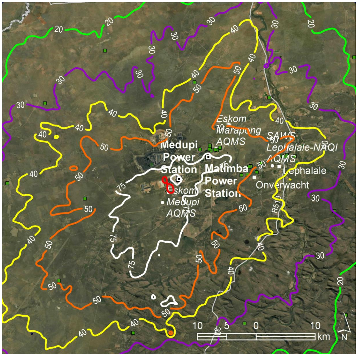
Figure 7-6: Predicted 99 th percentile 24-hour SO 2 concentrations in µg/m 3 resulting from emissions from Medupi: Scenario A (2025) (NAAQS limit 125 µg/m 3 )
