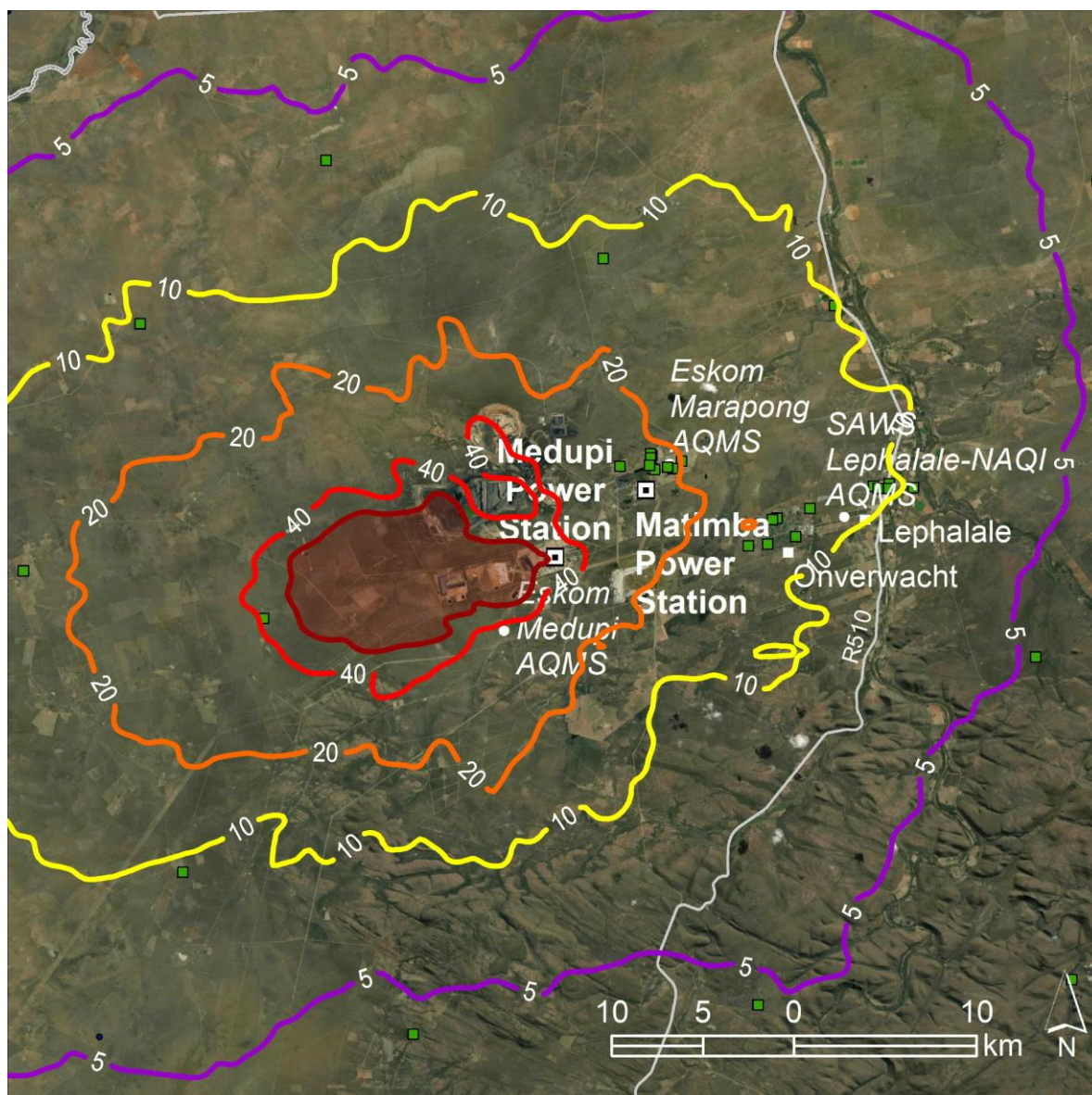
Figure 7-38: Predicted 99 th percentile of the 24-hour PM 2.5 concentrations in µg/m 3 resulting from emissions from Medupi: Scenario 1 (Current) (NAAQS limit 40 ug/m 3 )
