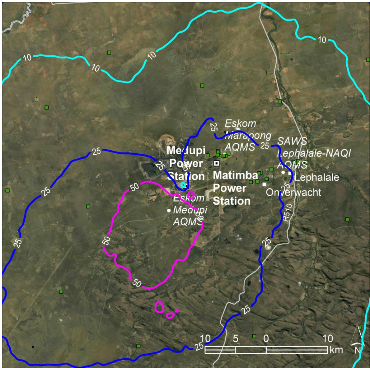
Figure 7-16: Predicted 99 th percentile 1-hour SO 2 concentrations in µg/m 3 resulting from emissions from Medupi: Scenario D (MES) (NAAQS limit 50 ug/m 3 )
