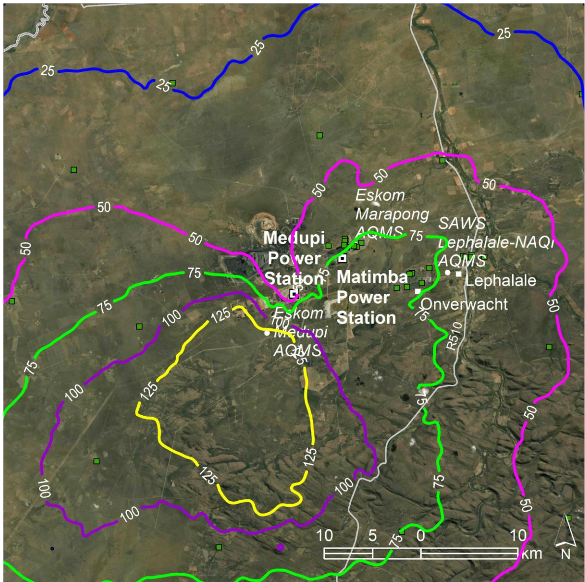
Figure 7-4: Predicted 99 th percentile 1-hour SO 2 concentrations in µg/m 3 resulting from emissions from Medupi: Scenario 1 (Current) (NAAQS limit 350 ug/m 3 )
