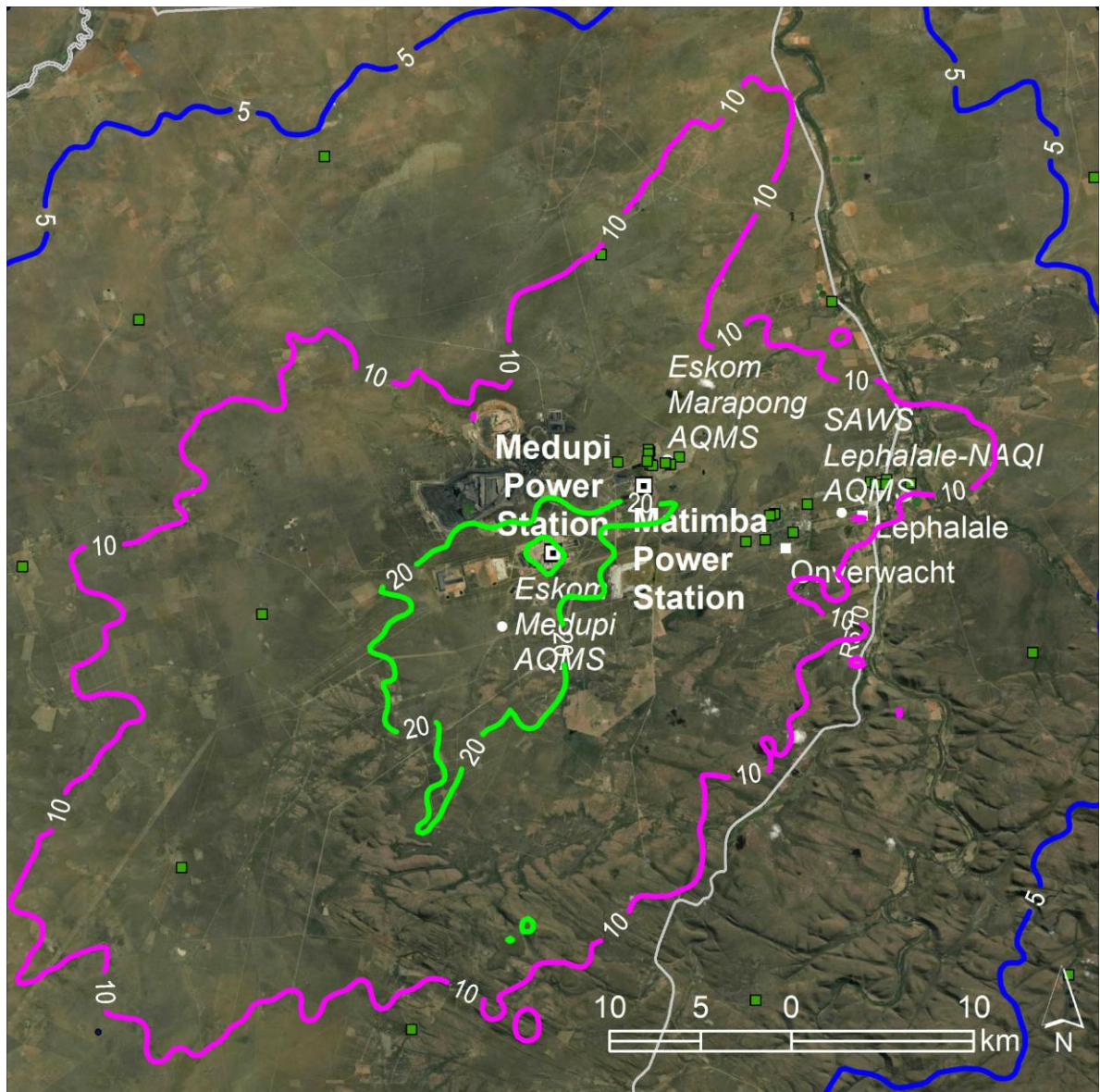
Figure 7-12: Predicted 99 th percentile 24-hour SO 2 concentrations in µg/m 3 resulting from emissions from Medupi: Scenario C (2036) (NAAQS limit 125 µg/m 3 )
