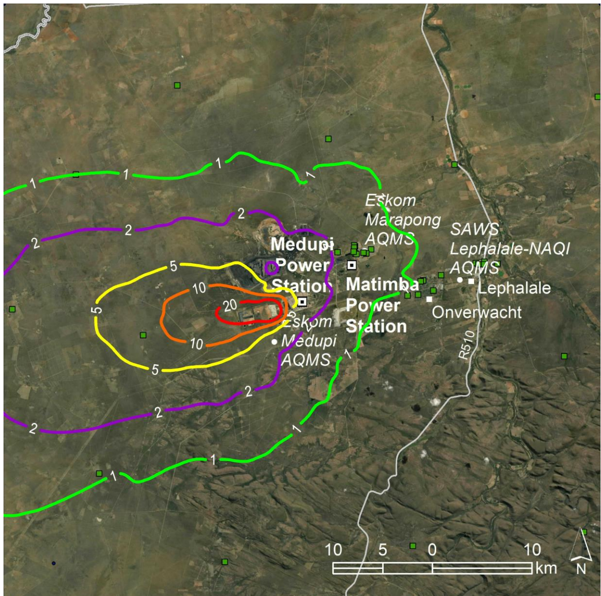
Figure 7-39: Predicted annual average PM 2.5 concentrations in µg/m 3 resulting from emissions from Medupi: Scenario A (2025) (NAAQS limit 20 ug/m 3 )
