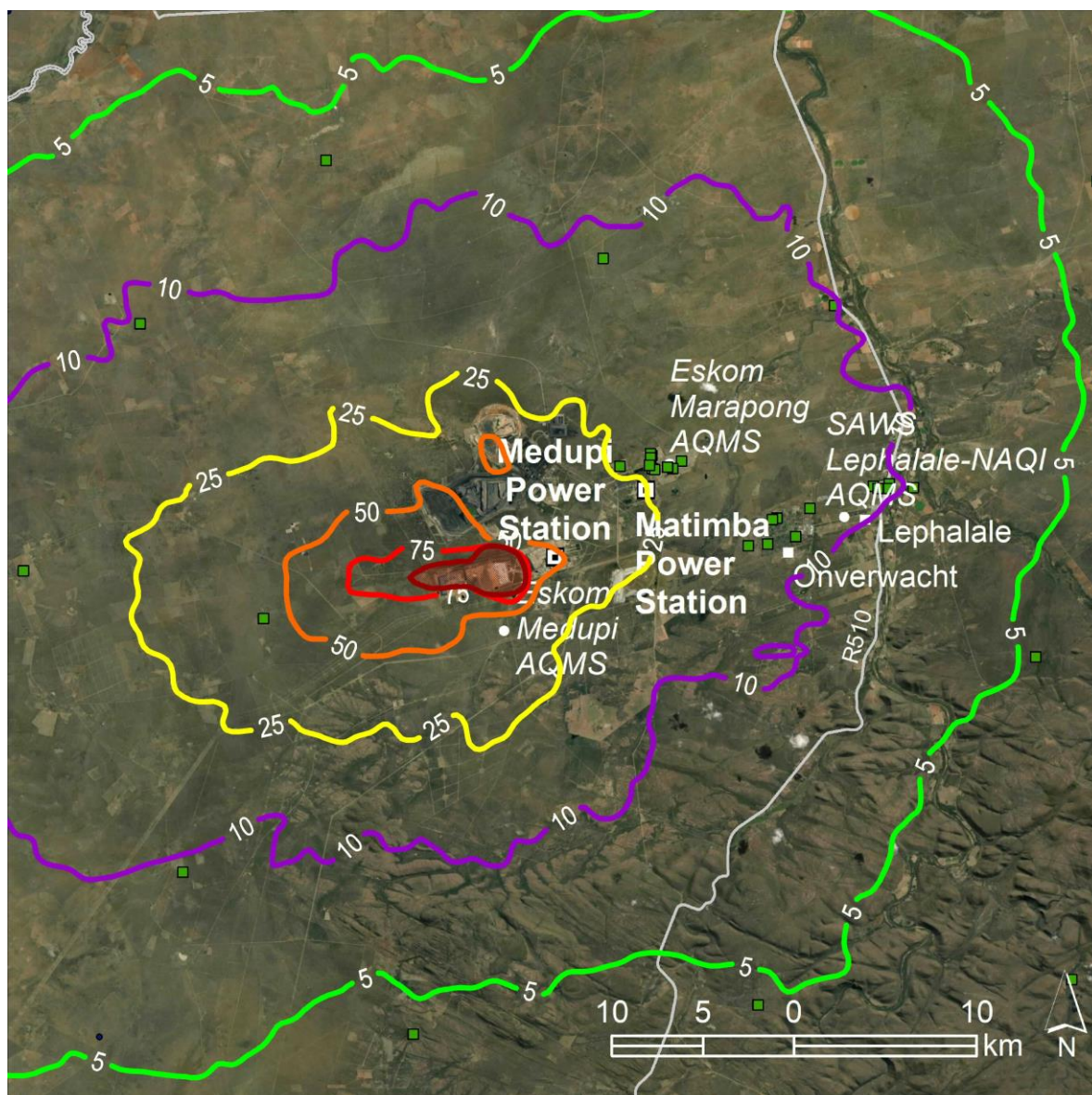
Figure 7-28: Predicted 99 th percentile of the 24-hour PM 10 concentrations in µg/m 3 resulting from emissions from Medupi: Scenario 1 (Current) (NAAQS limit 75 ug/m 3 )
