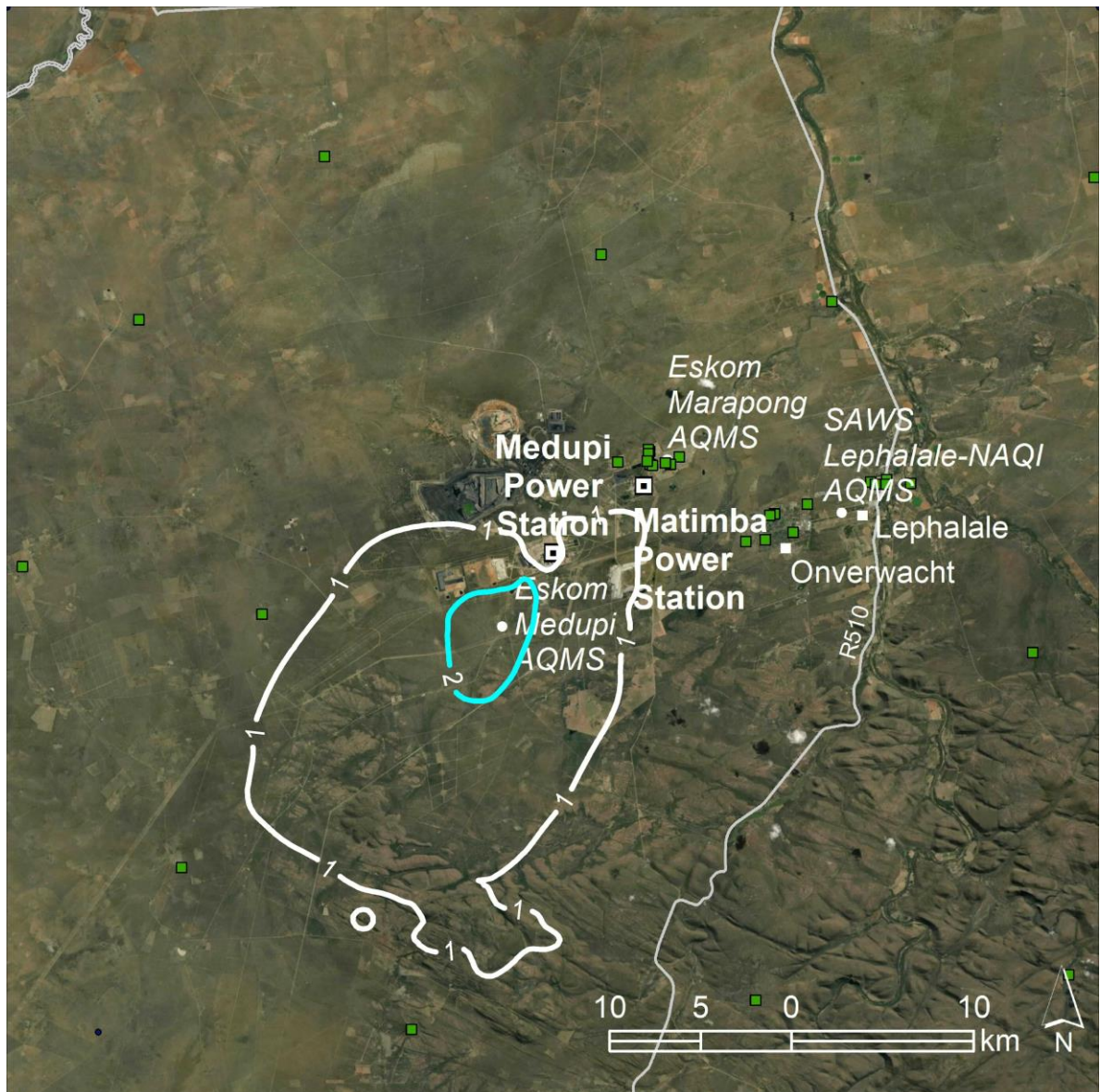
Figure 7-21: Predicted annual average NO 2 concentrations in µg/m 3 resulting from emissions from Medupi: Scenario B (2031) (NAAQS limit 40 ug/m 3 )
