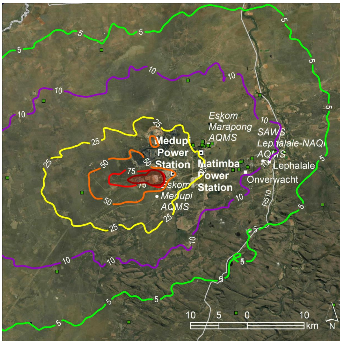
Figure 7-32: Predicted 99 th percentile of the 24-hour PM 10 concentrations in µg/m 3 resulting from emissions from Medupi: Scenario B (2031) (NAAQS limit 75 ug/m 3 )
