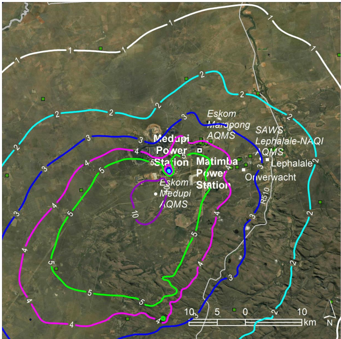
Figure 7-8: Predicted annual average SO 2 concentrations in µg/m 3 resulting from emissions from Medupi: Scenario B (2031) (NAAQS limit 50 ug/m 3 )
