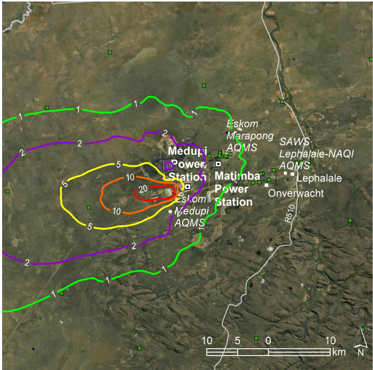
Figure 7-37: Predicted annual average PM 2.5 concentrations in µg/m 3 resulting from emissions from Medupi: Scenario 1 (Current) (NAAQS limit 20 µg/m 3 )
