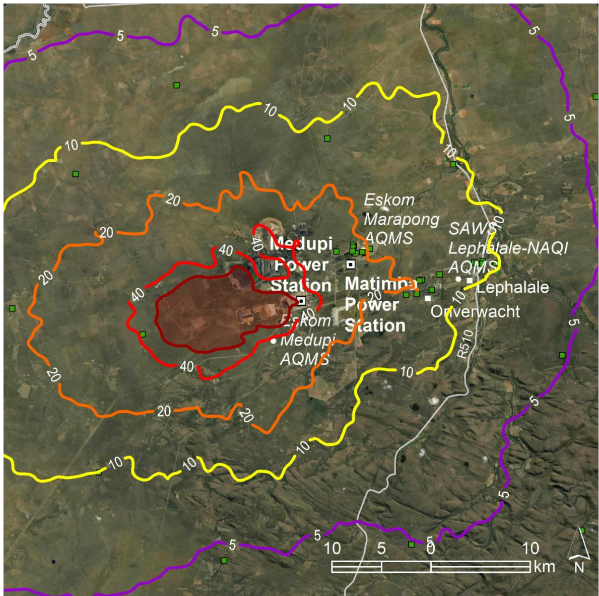
Figure 7-40: Predicted 99 th percentile of the 24-hour PM 2.5 concentrations in µg/m 3 resulting from emissions from Medupi: Scenario A (2025) (NAAQS limit 40 µg/m 3 )
