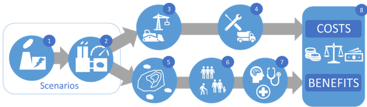
Figure 7-1 – APHR-BCA Methodology
