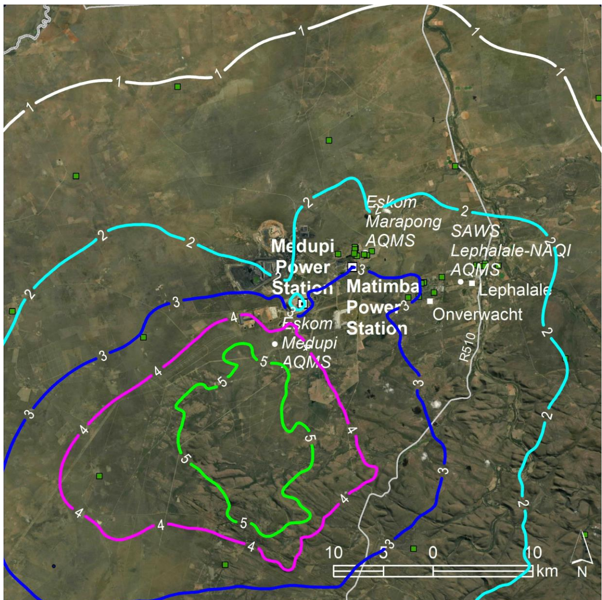
Figure 7-2: Predicted annual average SO 2 concentrations in µg/m 3 resulting from emissions from Medupi: Scenario 1 (Current) (NAAQS limit 50 ug/m 3 )
