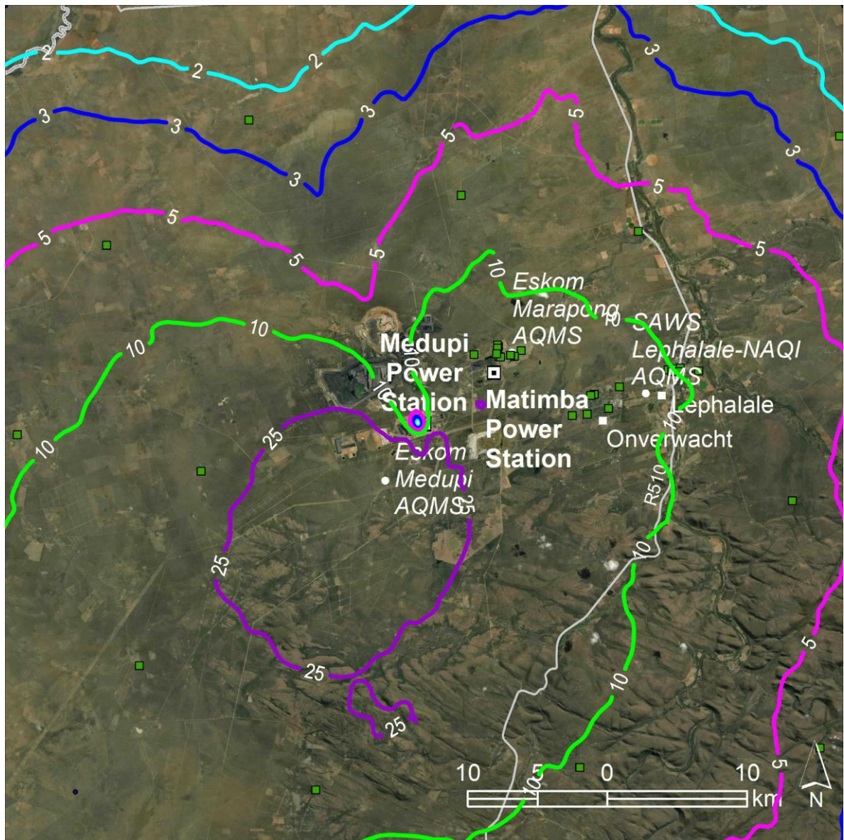
Figure 7-24: Predicted 99 th percentile 1-hour NO 2 concentrations in µg/m 3 resulting from emissions from Medupi: Scenario C (2036) (NAAQS limit 200 µg/m 3 )
