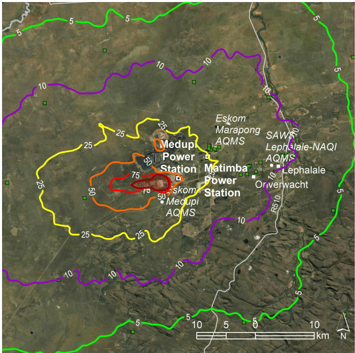
Figure 7-30: Predicted 99 th percentile of the 24-hour PM 10 concentrations in µg/m 3 resulting from emissions from Medupi: Scenario A (2025) (NAAQS limit 75 ug/m 3 )
