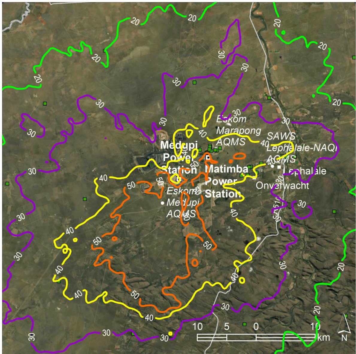
Figure 7-3: Predicted 99 th percentile 24-hour SO 2 concentrations in µg/m 3 resulting from emissions from Medupi: Scenario 1 (Current) (NAAQS limit 125 ug/m 3 )
