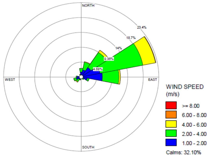
Figure 6-2: Annual windrose at the Medupi AQMS
