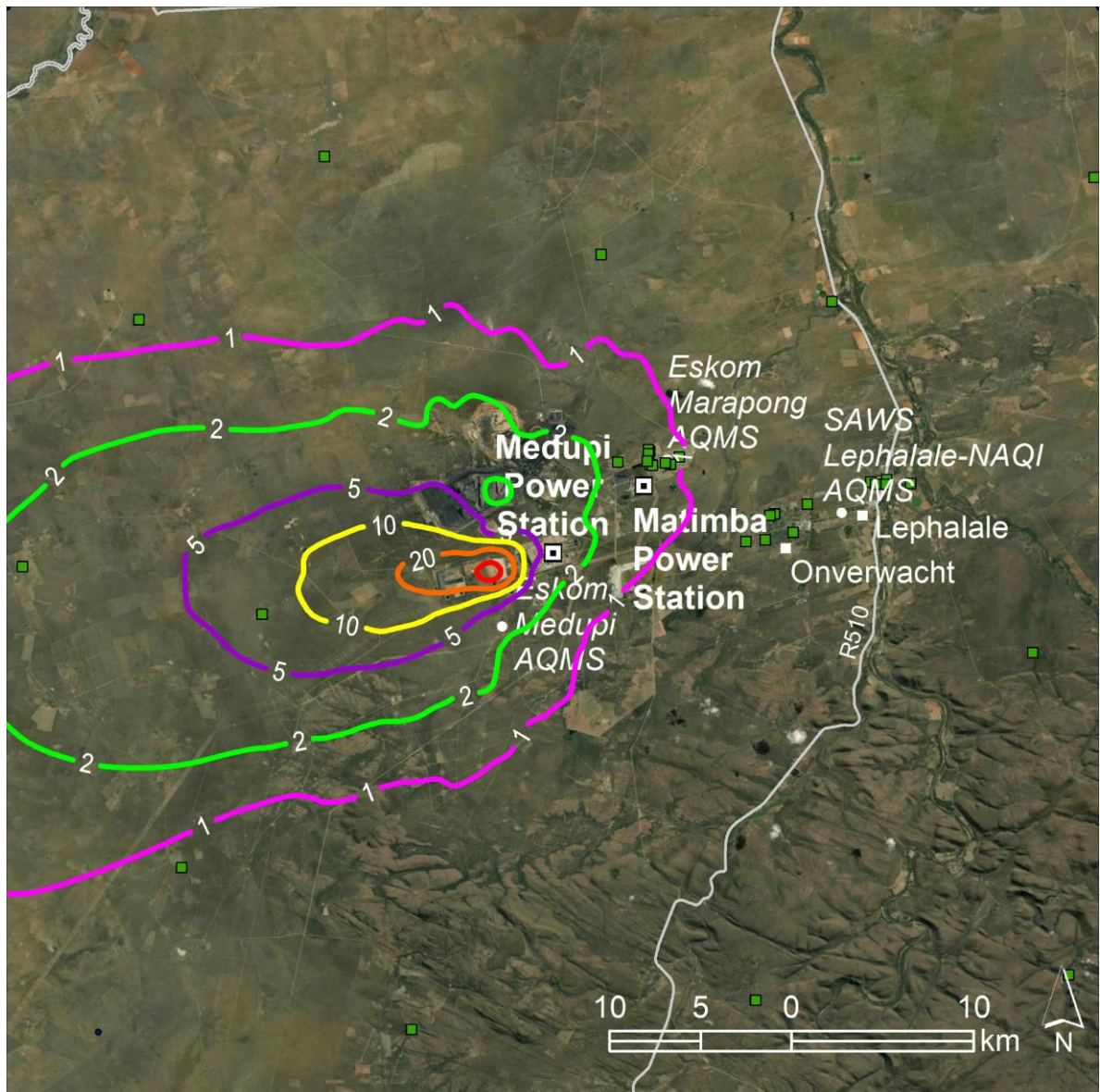
Figure 7-33: Predicted annual average PM 10 concentrations in µg/m 3 resulting from emissions from Medupi: Scenario C (2036) (NAAQS limit 40 µg/m 3 )
