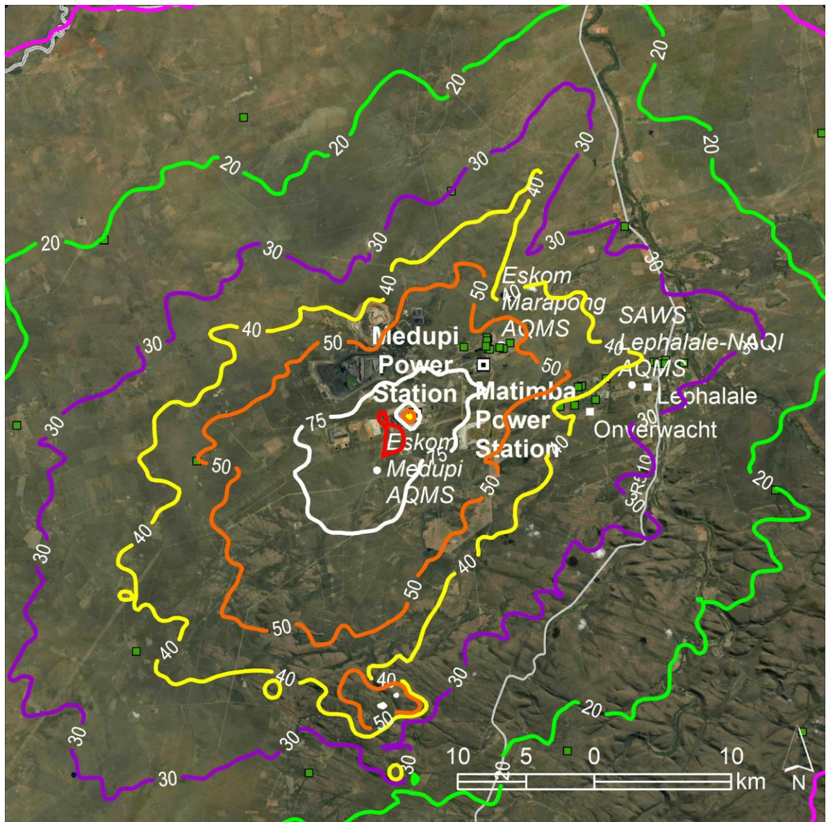
Figure 7-9: Predicted 99 th percentile 24-hour SO 2 concentrations in µg/m 3 resulting from emissions from Medupi: Scenario B (2031) (NAAQS limit 125 µg/m 3 )
