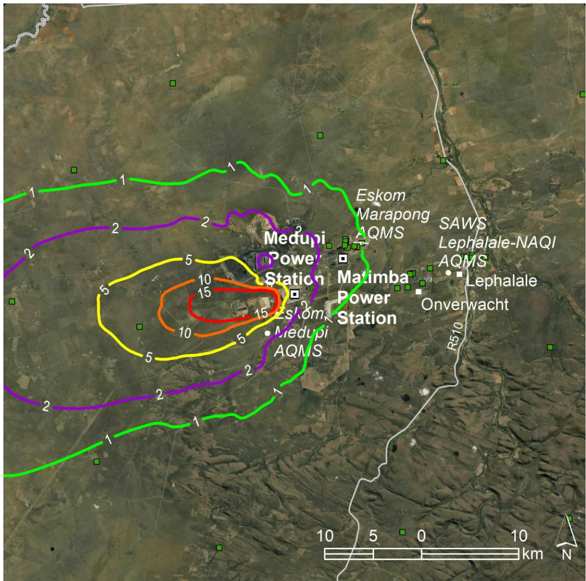
Figure 7-43: Predicted annual average PM 2.5 concentrations in µg/m 3 resulting from emissions from Medupi: Scenario C (2036) (NAAQS limit 15 ug/m 3 )
