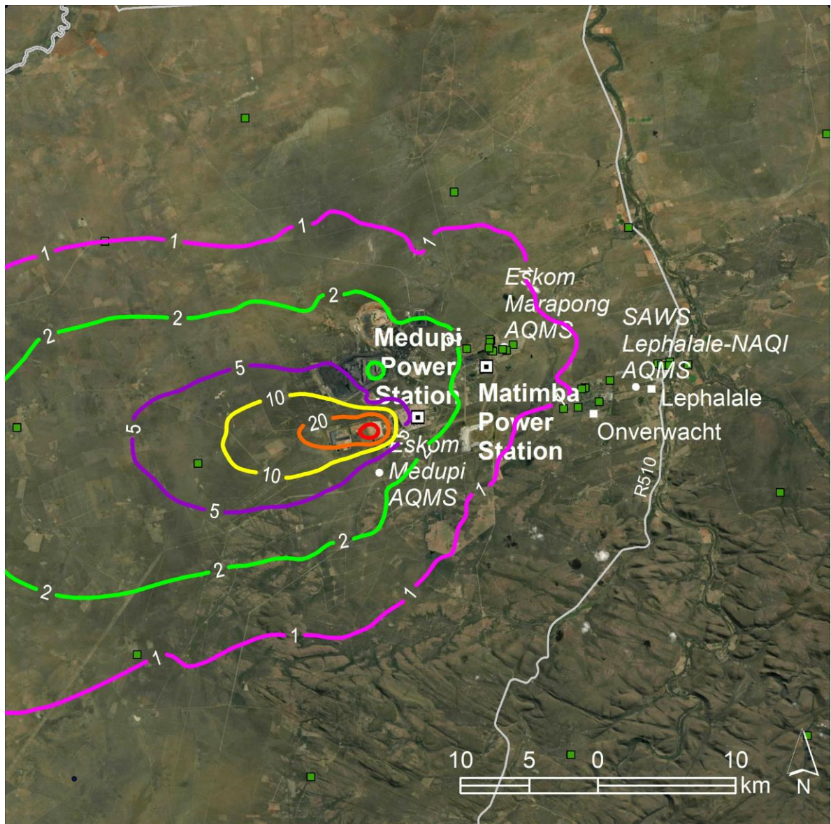
Figure 7-29: Predicted annual average PM 10 concentrations in µg/m 3 resulting from emissions from Medupi: Scenario A (2025) (NAAQS limit 40 ug/m 3 )
