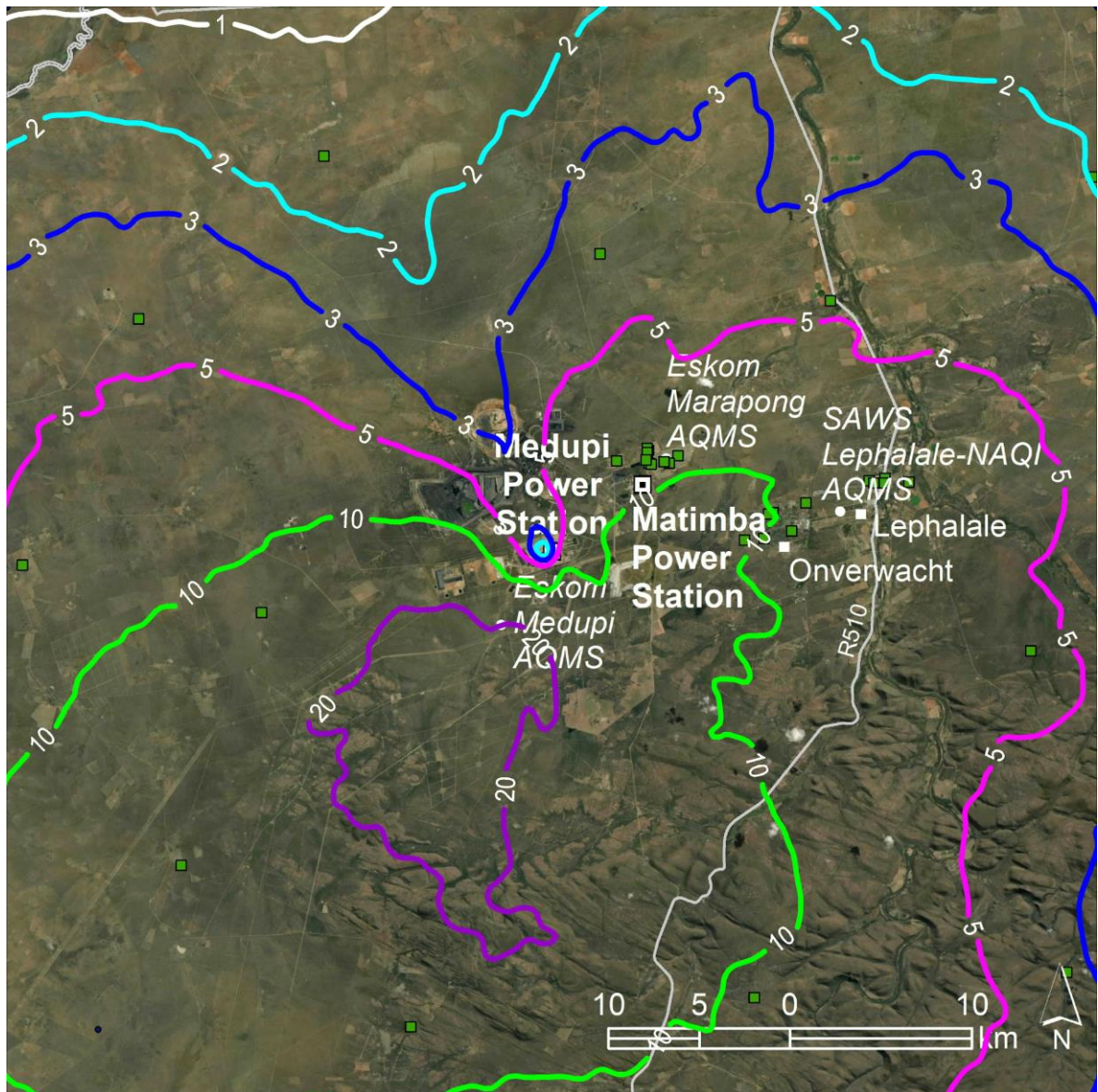
Figure 7-18: Predicted 99 th percentile 1-hour NO 2 concentrations in µg/m 3 resulting from emissions from Medupi: Scenario 1 (Current) (NAAQS limit 200 ug/m 3 )
