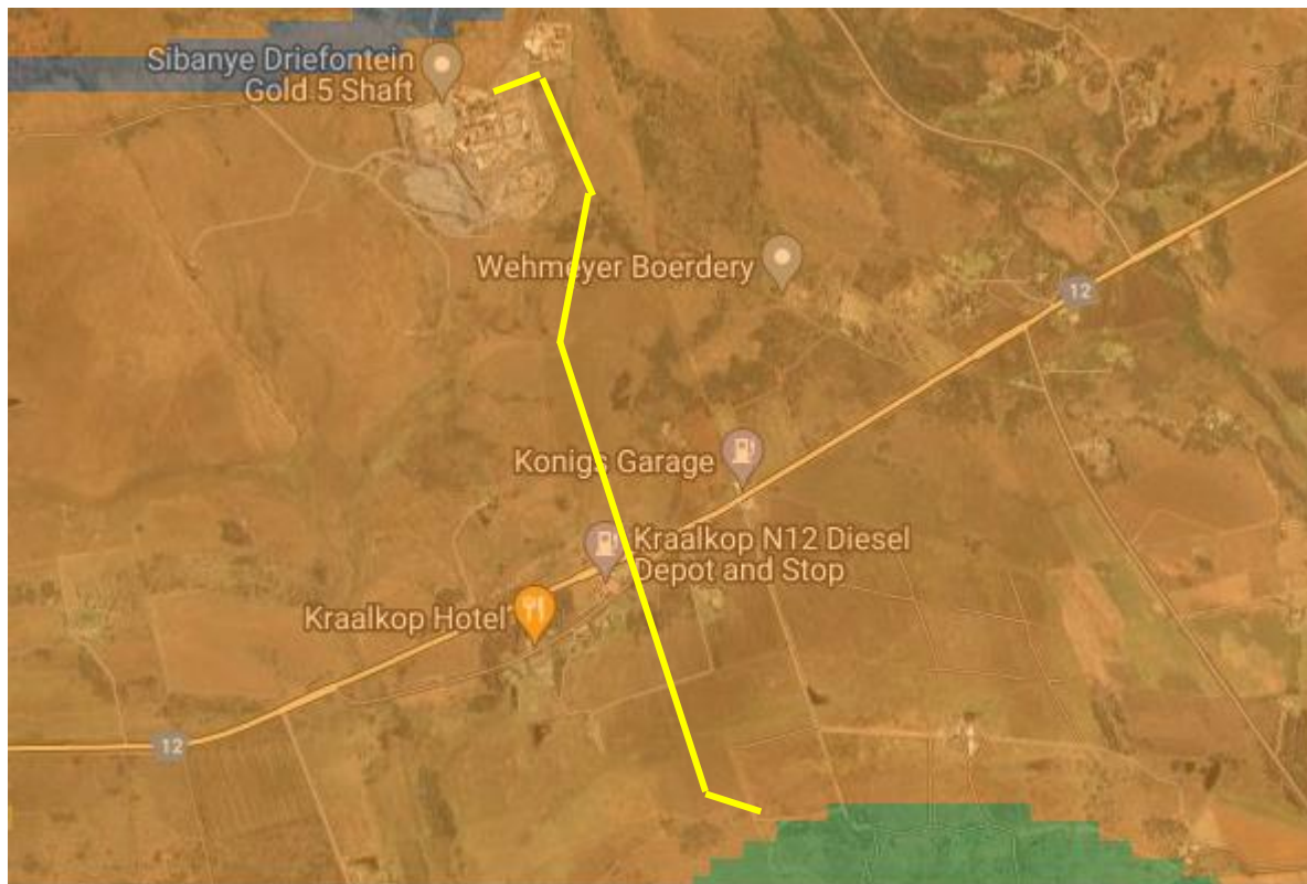
Figure 4: SAHRIS palaeosensitivity map for the site for the proposed Igolide WEF EGI route indicated by the yellow line. Background colours indicate the following degrees of sensitivity: red = very highly sensitive; orange/yellow = high; green = moderate; blue = low; grey = insignificant/zero.
