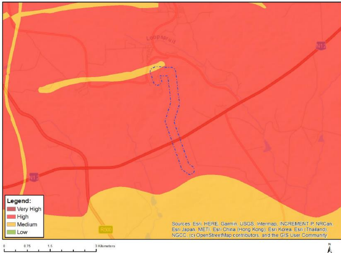
Figure 5: DFFE Screening palaeosensitivity map for the Igolide WEF EGI route. Colours as indicated. Note that highly sensitive = dark orange in DFFE and light orange in SAHRIS, and moderately sensitive = yellow in DFFE and green in SAHRIS maps. The sensitivities are incorrect and should only be moderately sensitive , not highly sensitive, because there are no fossils.
