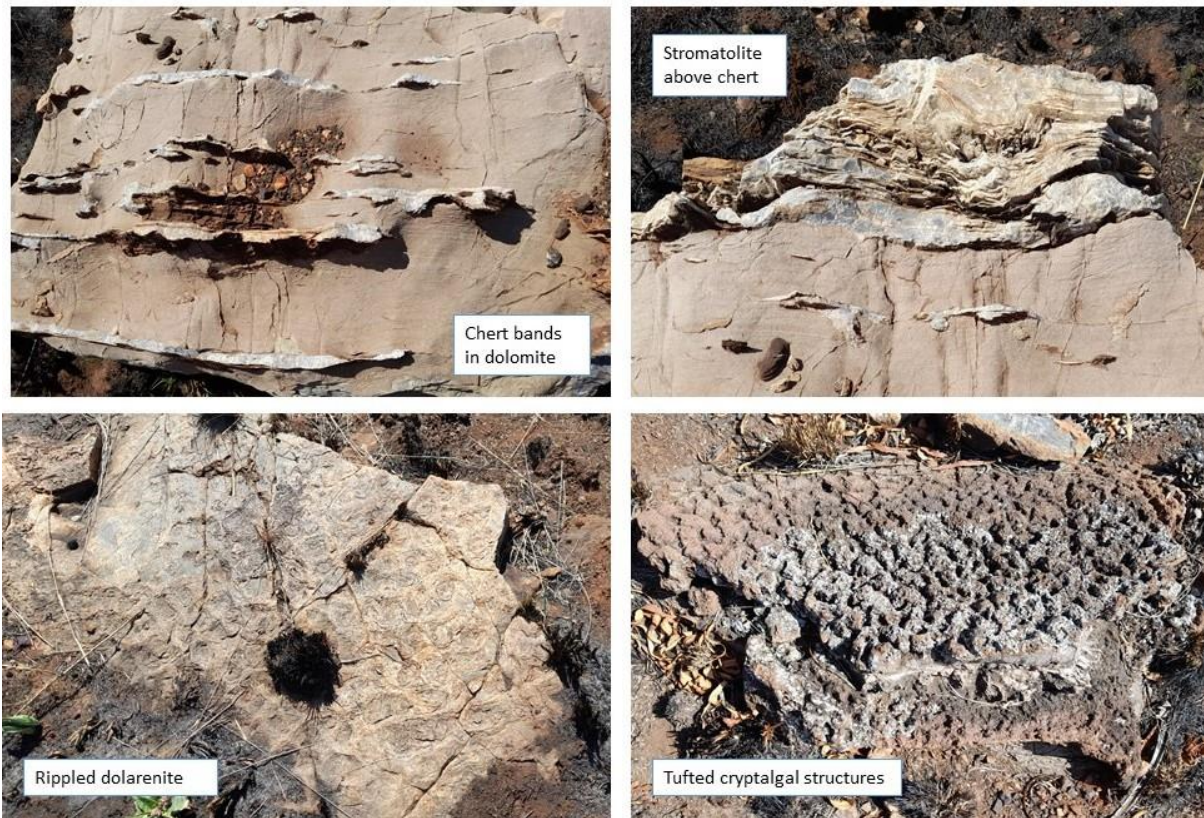
Figure 8: Photographs of stromatolites as seen in the field.
