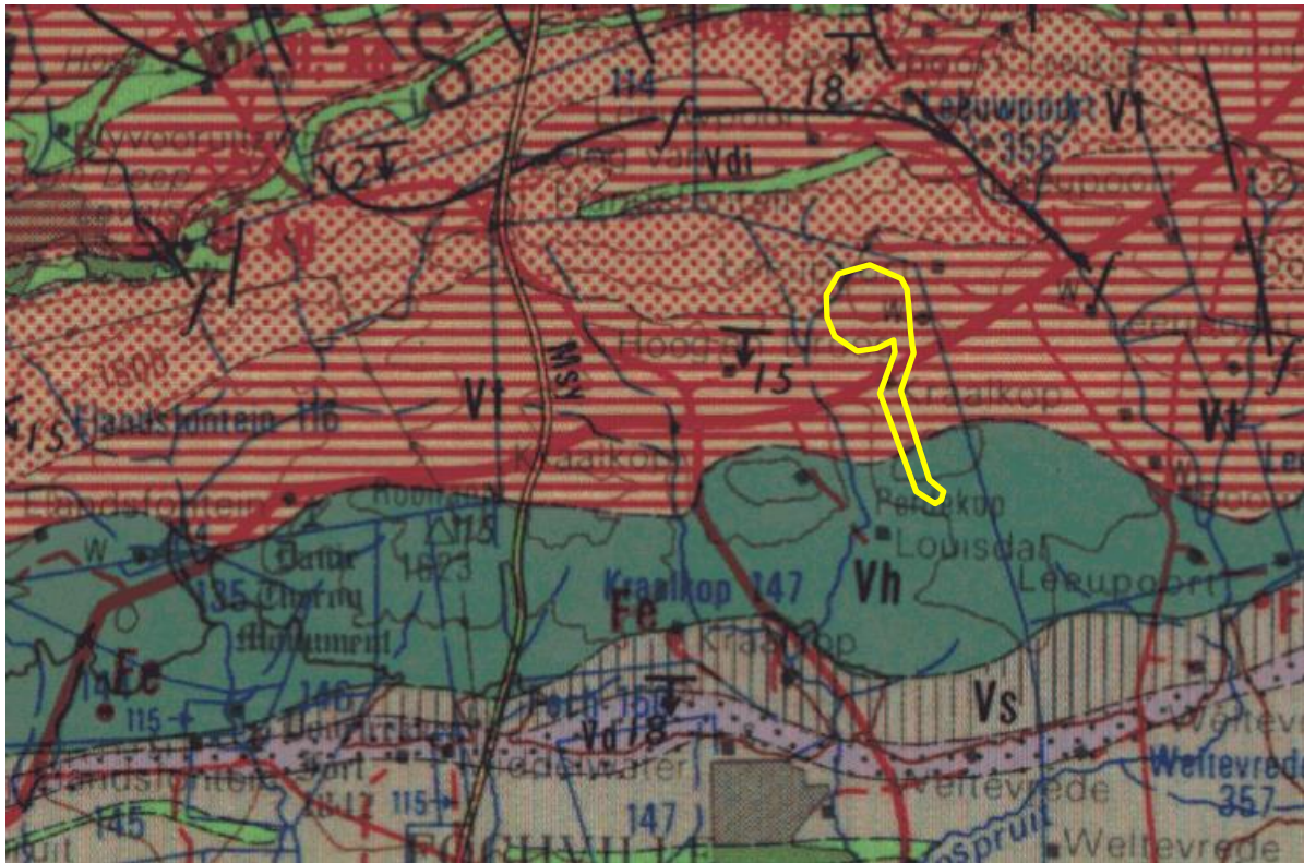
Figure 3: Geological map of the area around the proposed Igolide EGI with the route indicated by the yellow line. Abbreviations of the rock types are explained in Table 4. Map enlarged from the Geological Survey 1: 250 000 map 2626 West Rand.
