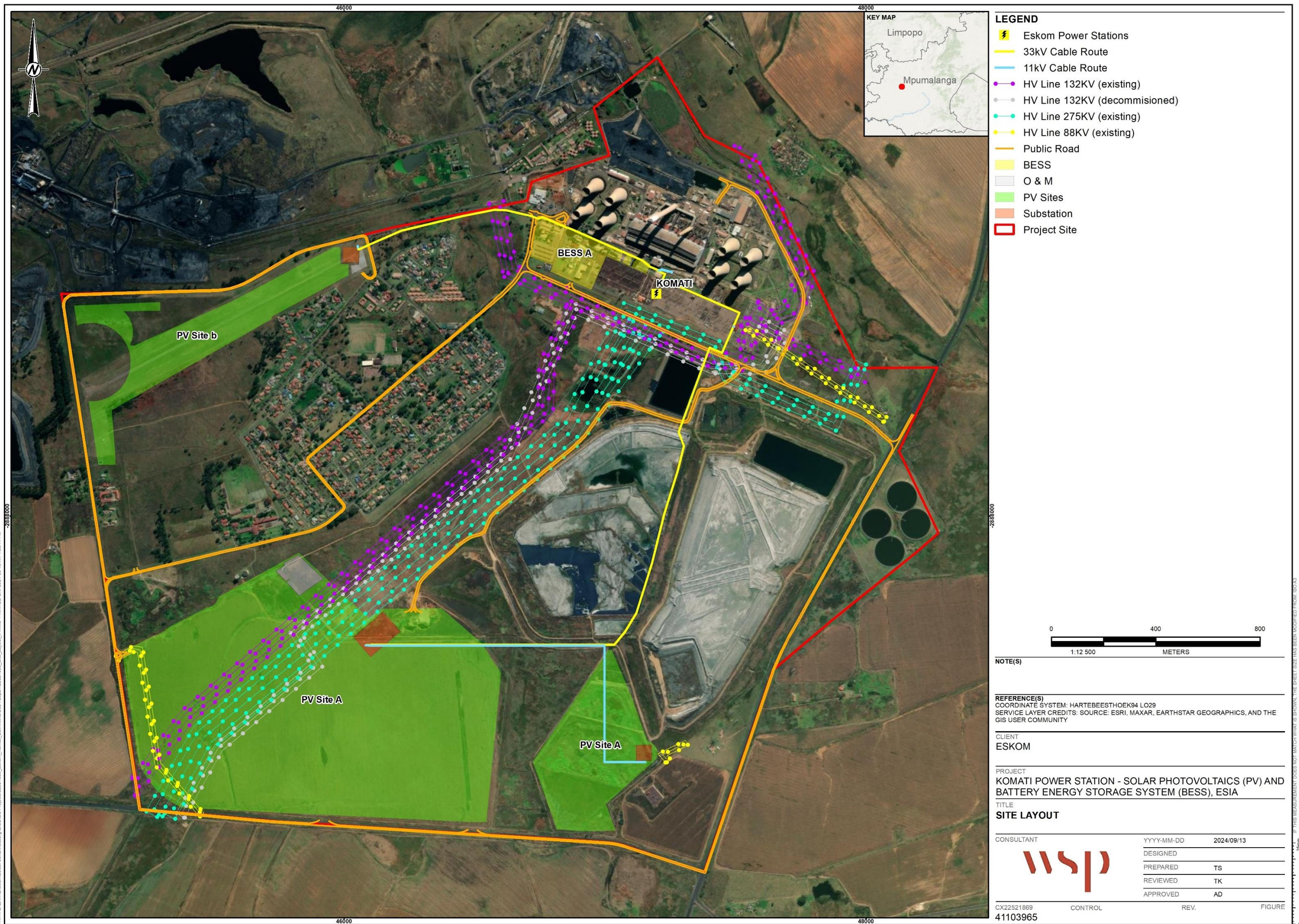
Figure 1: Proposed Komati Solar PV and BESS Facility and associated infrastructure.
