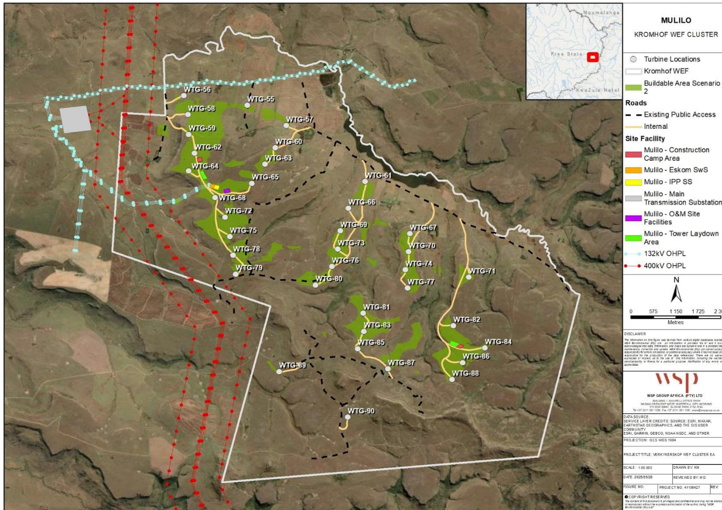
Figure 4-2 - Positions of the Turbines
