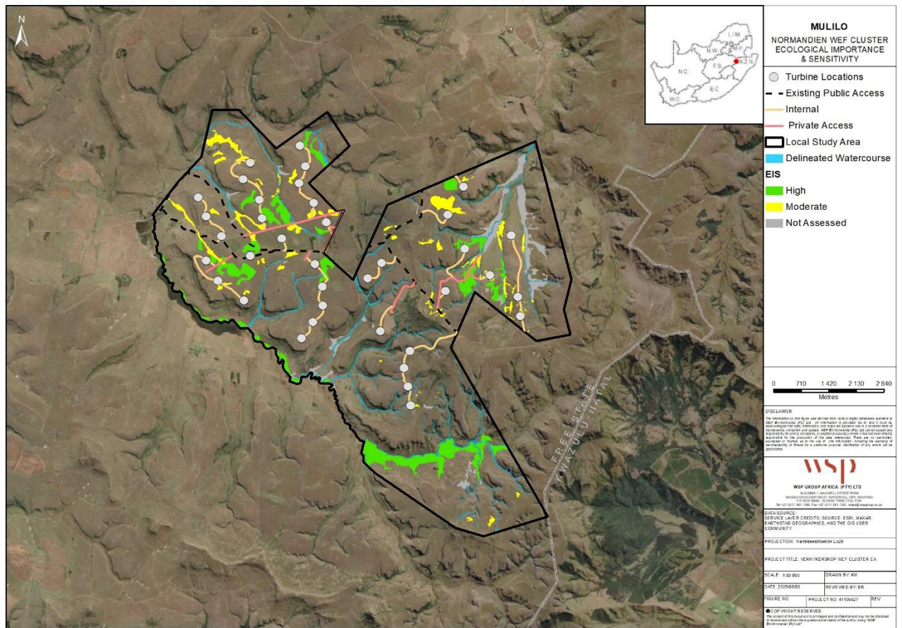
Figure 6-7 - IS of the wetlands within the Normandien project area
