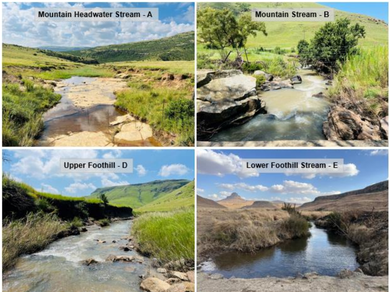
Figure 6-9 – Representative photos of the riverine geomorphological zones and physical conditions of rivers within the PAOI. Letters A-E represent the zone classes
