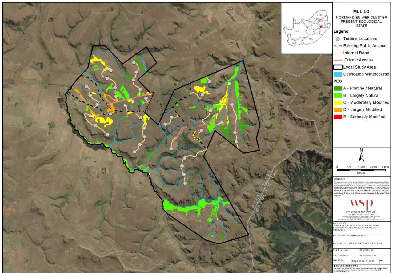
Figure 6-6 - PES of the wetlands within the Normandien project area
