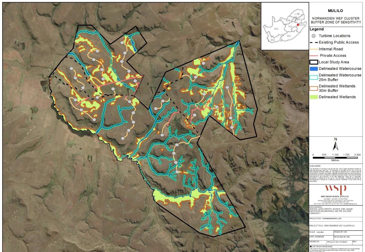
Figure 8-2 - Map showing recommended buffers width for riparian and wetland habitats
