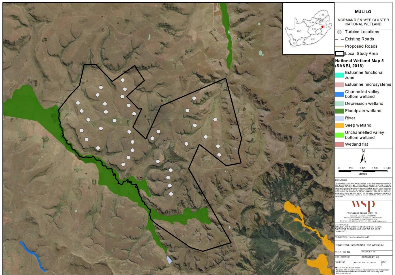
Figure 5-5 - National Wetland Map 5 for the proposed Normandien project area
