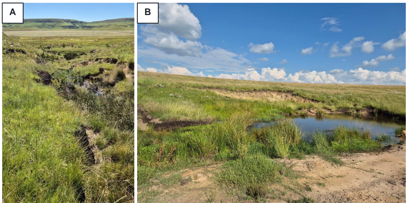
Figure 6-3 - Typical Channelled Valley Bottom (CVB) wetland habitats (A and B) observed within the proposed Normandien project footprint
