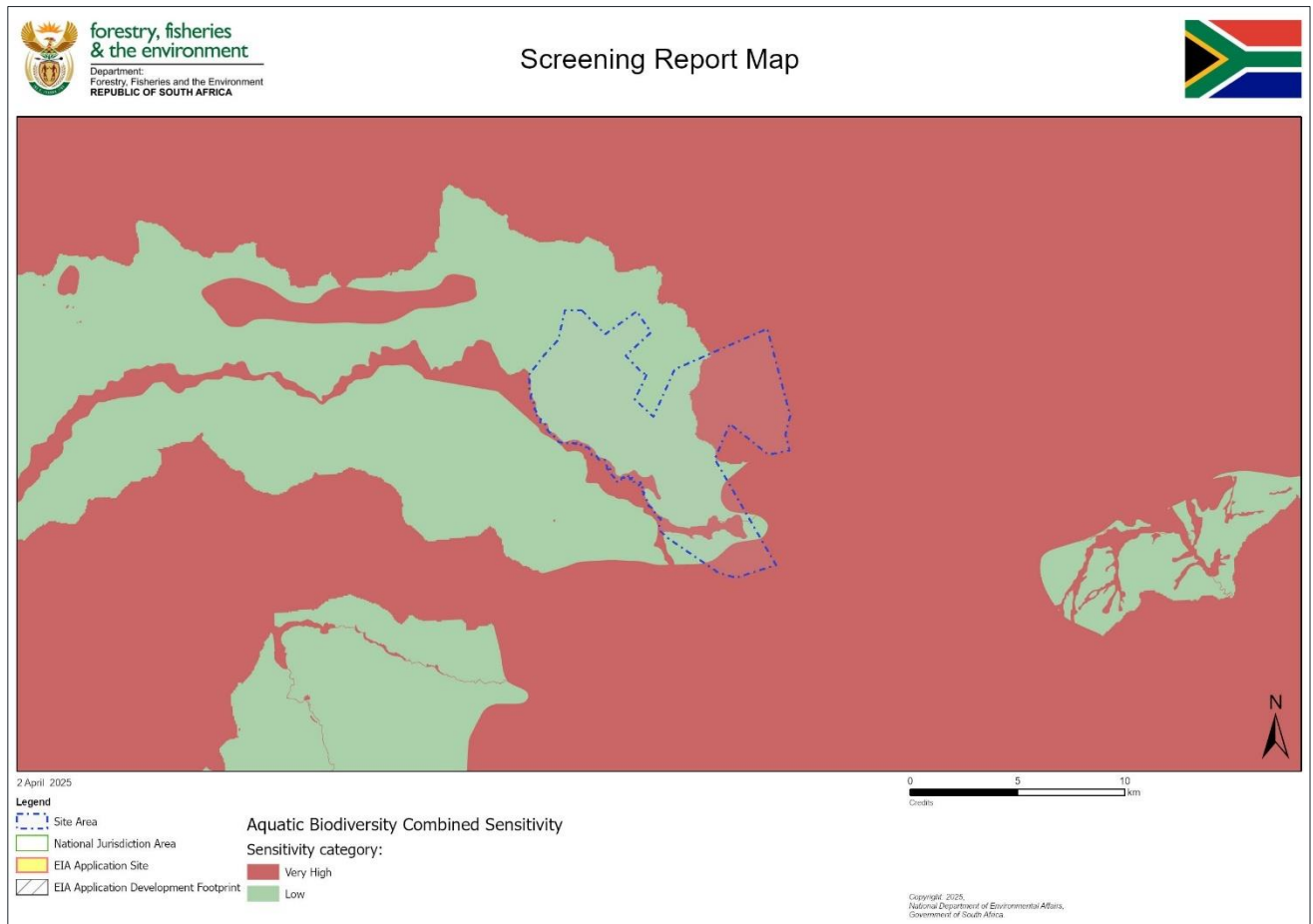
Figure 3-3 – Study area in relation to the DFFE web-based Environmental Screening Tool
