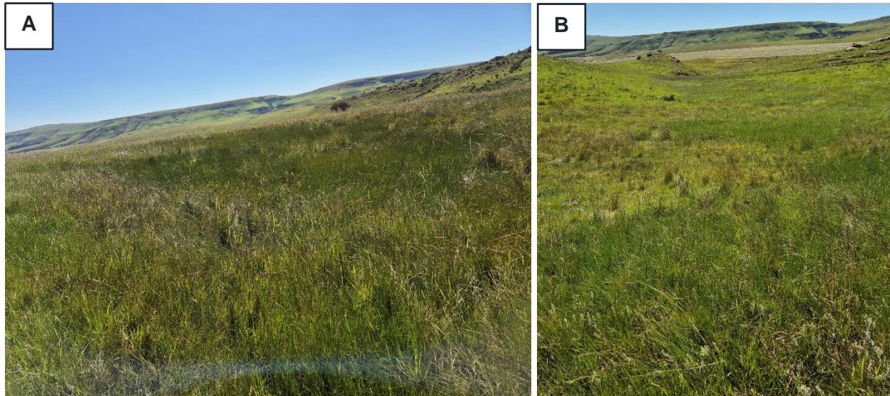
Figure 6-4 - Typical Unchanneled Valley Bottom (UVB) wetland habitats (A and B) observed within the proposed Normandien project footprint
