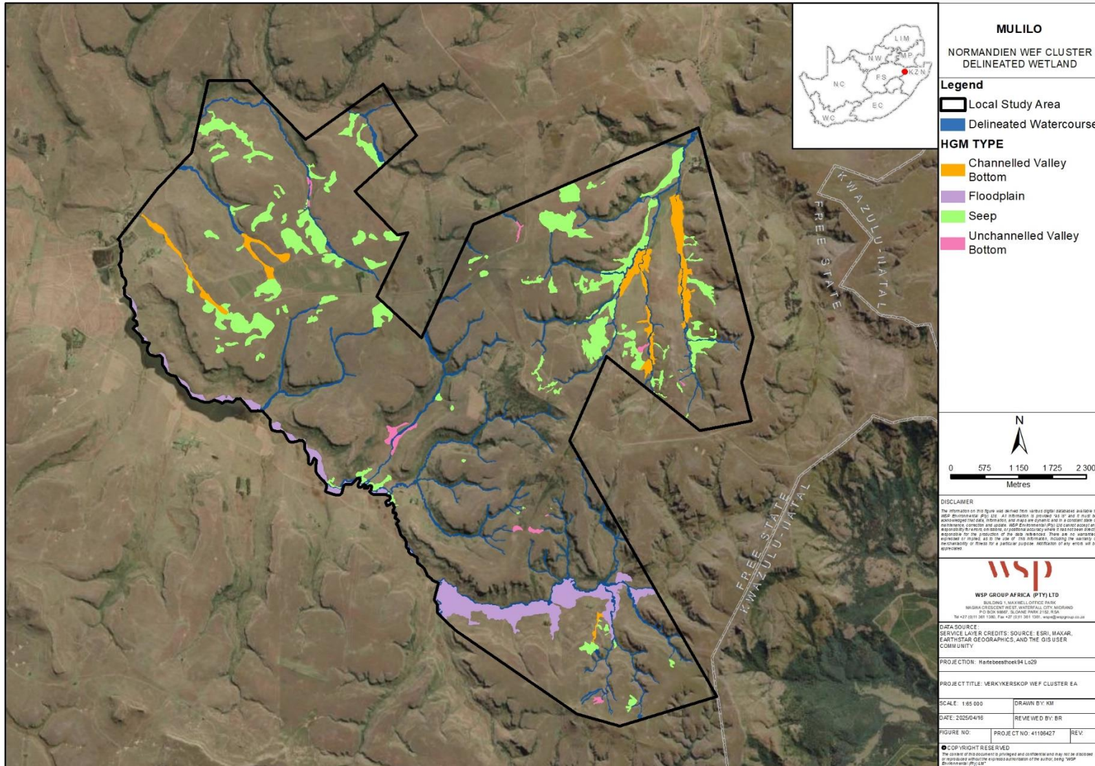
Figure 6-1 - Extent and classification of wetland HGM units identified within the proposed Normandien project boundary
