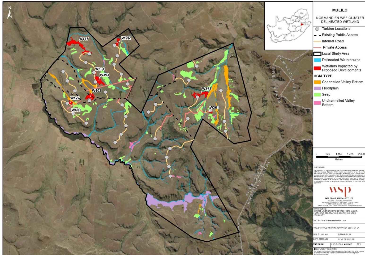
Figure 8-3 - Identified wetlands that will be impacted by the proposed Normandien WEF infrastructure development
