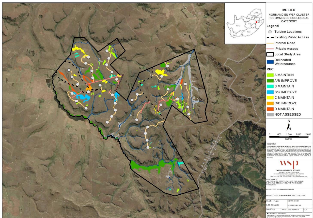
Figure 6-8 - The RECs for the wetlands within the Normandien study area
