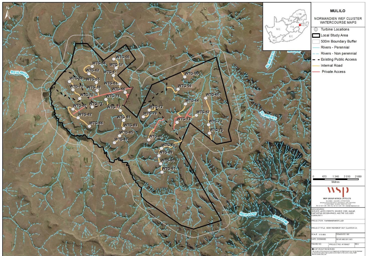
Figure 3-2 - Normandien WEF Project Area of Influence
