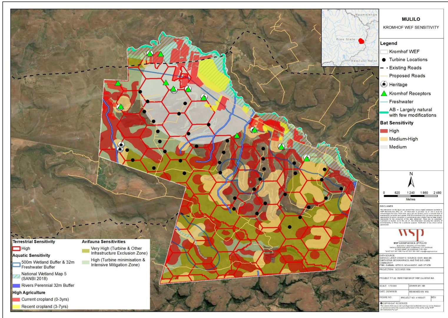
Figure 7-1 - Kromhof WEF – Consolidated Site Sensitivity Map overlain by Preliminary Project Layout
