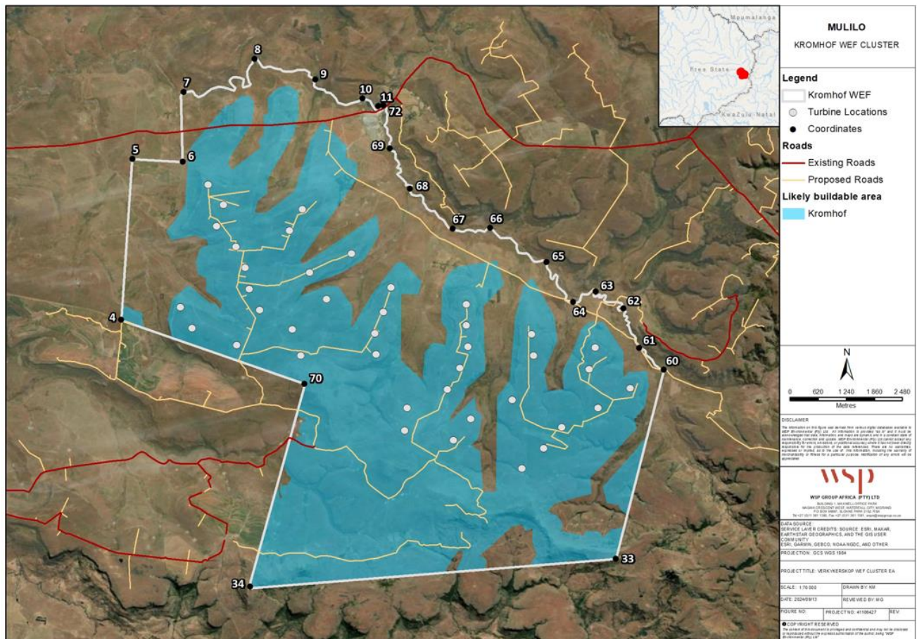
Figure 3-1 - Preliminary Layout and Coordinates of the boundary of the properties associated with the proposed Kromhof WEF
