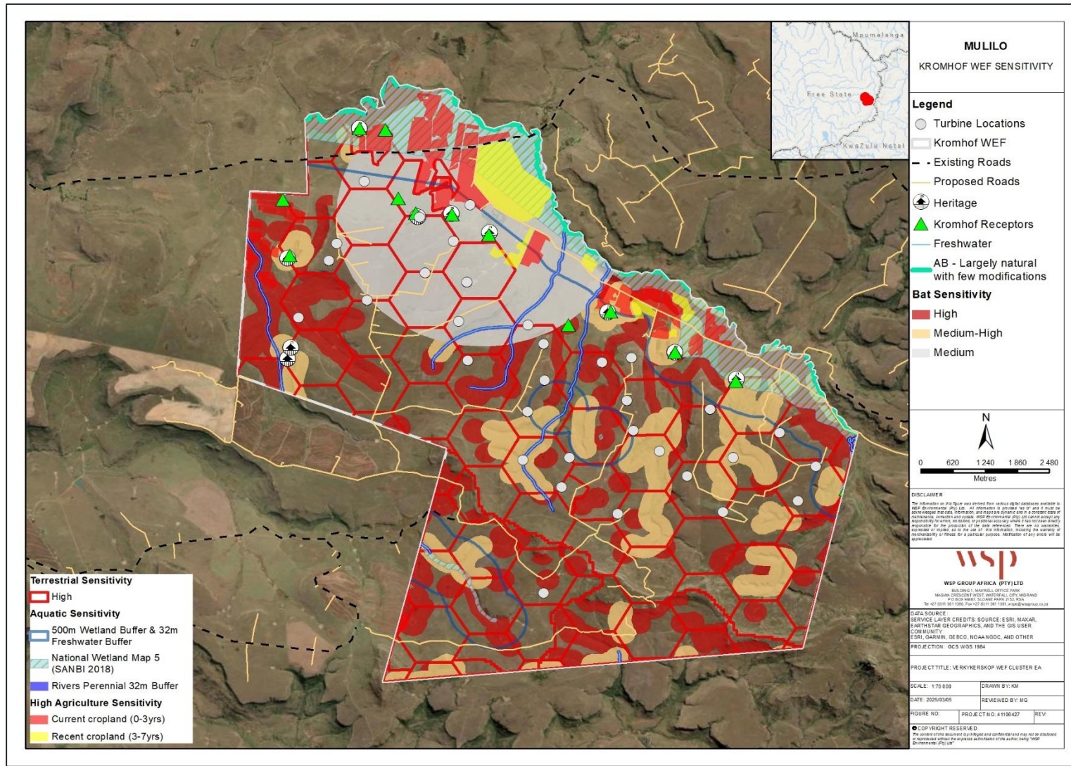
Figure 7-3 - Kromhof WEF - Map illustrating the Optimised Layout (excluding avifauna)
