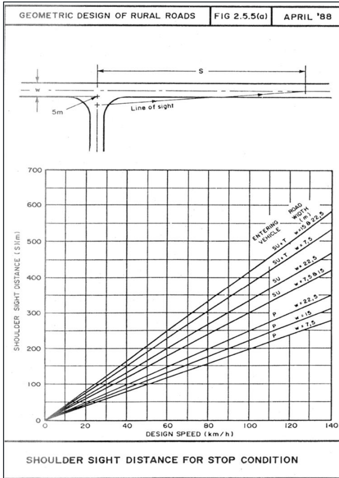
Figure 6-37 - Shoulder sight distance (TRH17)
