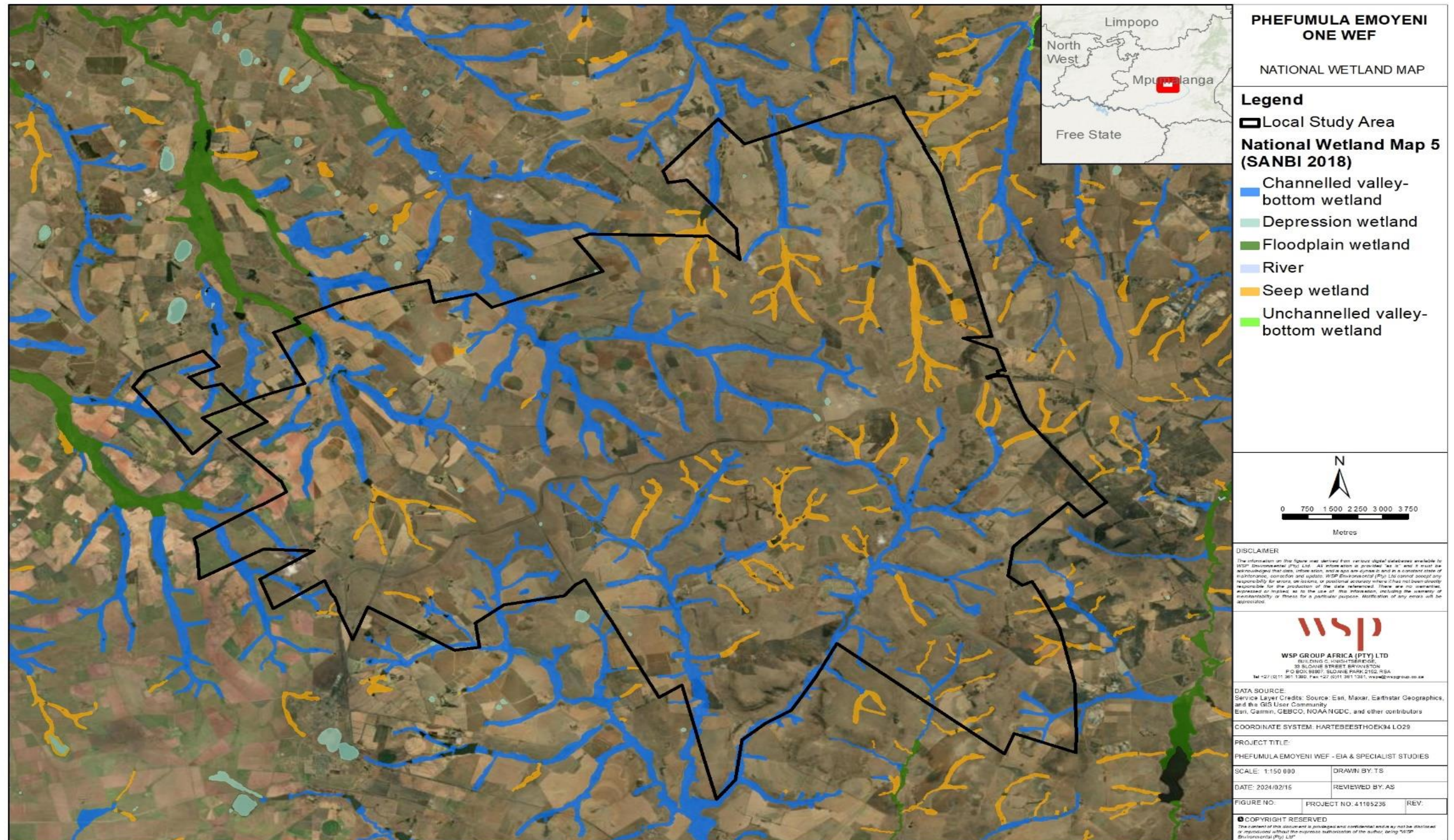
Figure 4-2 - NFEPA Wetlands
