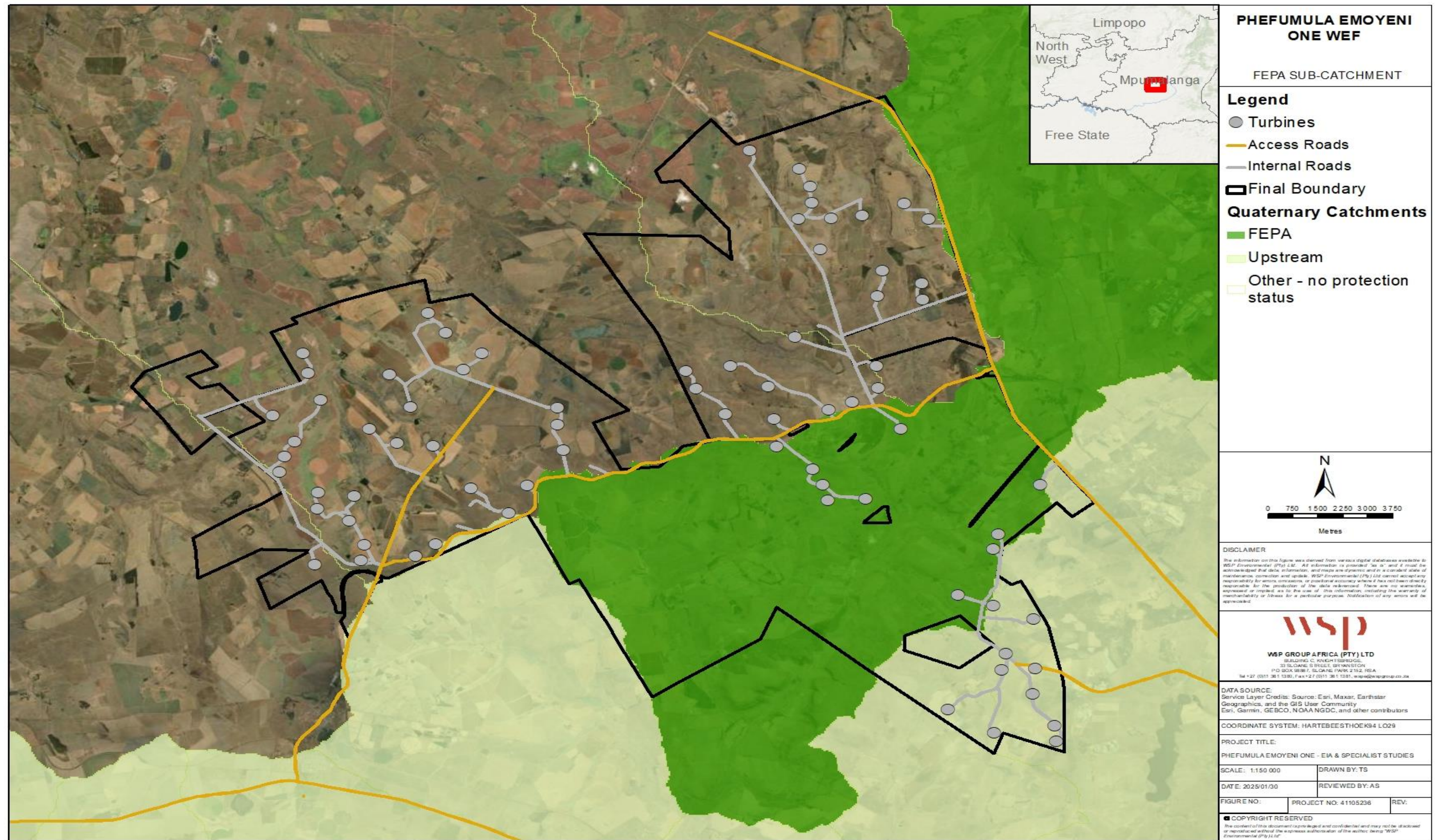
Figure 4-1 - FEPA Sub-Catchment
