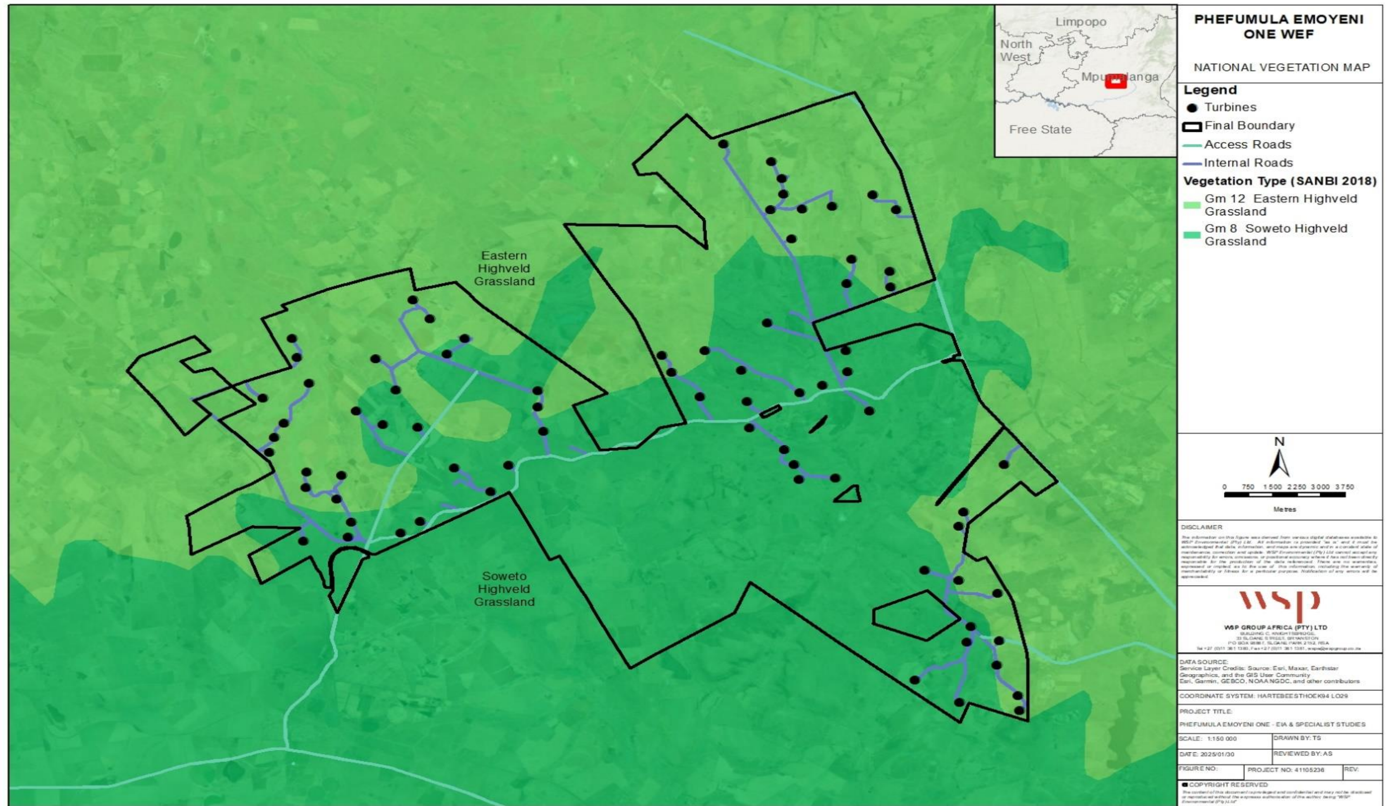
Figure 3-5 - Vegetation Types
