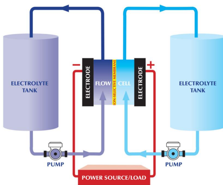
FIGURE 3.2.1.1 – Schematic Diagrams of Redox Flow BESS
