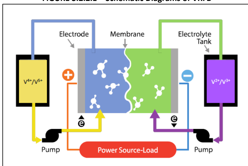
FIGURE 3.2.2.1 – Schematic Diagrams of VRFB
